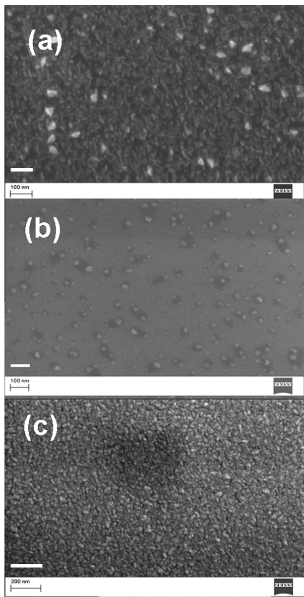
Fig. 1. SEM images of the ZnO-based films: (a) ZnO-1, (b) ZnO-2, (c) ZnO-3.
