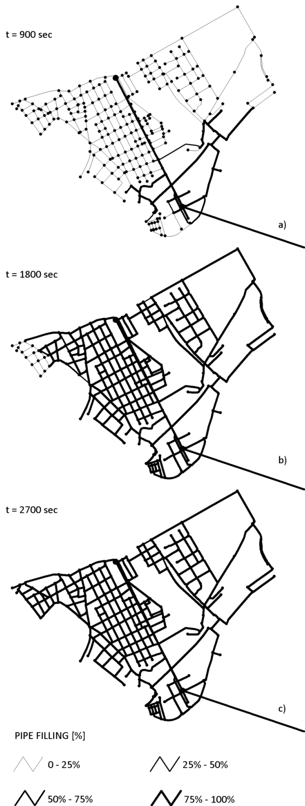
Figure 7. Dynamics of pipe filling in the network
