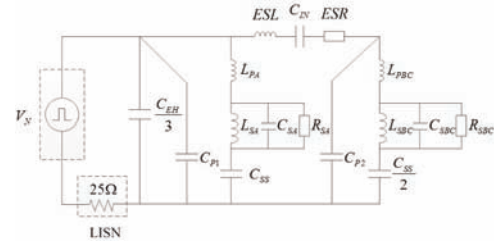
Fig.2 CM equivalent circuit considering the near-field coupling
