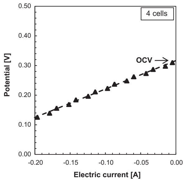
Fig. 8. Cyclic voltammery galvanostatic on a stack equipped with four cells. Stack equipped with 450 \mu\text{m} spacers in electrode/central compartments; flow rate in single channel: 13 mL/min.
