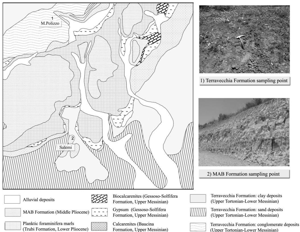
Figure 2. Lithologic map of the area between Monte Polizzo and Salemi.
