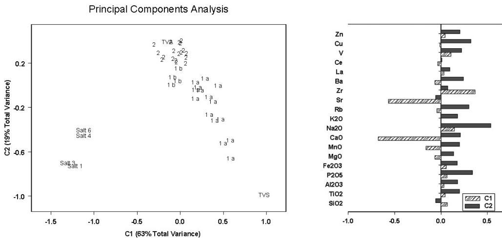
Figure 8. Plot of PCA scores in the plane of the first two principal components C1 and C2 concerning the ceramic samples belonging to the PCRUs 1a, 1b, 2, the MAB Formation clays (SALT 1, SALT 3, SALT 4, SALT 6) and the Terravecchia Formation clays (TVA= SALT 11; TVS = SALT 10). Histogram at the right shows the loadings of chemical variables on the two considered principal components.
