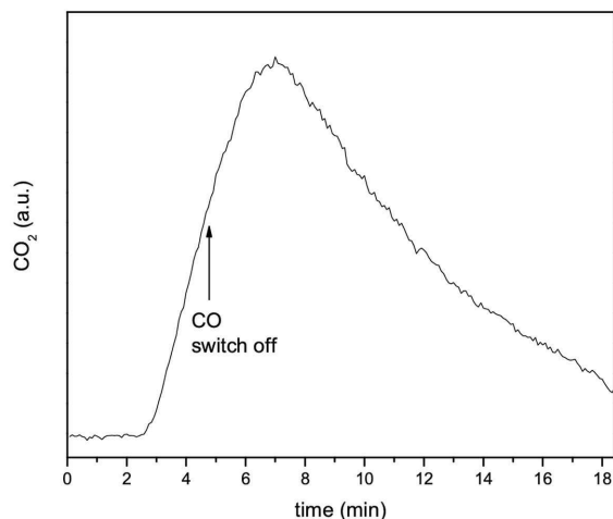
Figure 5 Kinetics of the CO 2 production at 773 K detected with the mass spectrometer during a 5 min CO flow. The switch-off time is indicated by the arrow.
