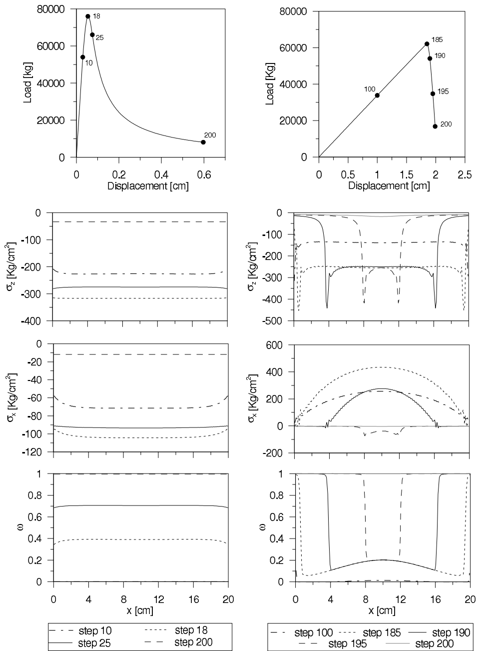
Figure 4: Uniaxial compression test of a masonry block. First coloumn: results for the case E_b = 10E_m ; second coloumn: results for the case E_m = 30E_b .
