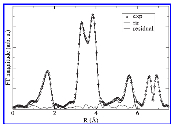
Figure 6. Fourier-transformed Zr K-edge EXAFS data (circles), best fit (thick line), and residual (thin line) of undoped BZ.
