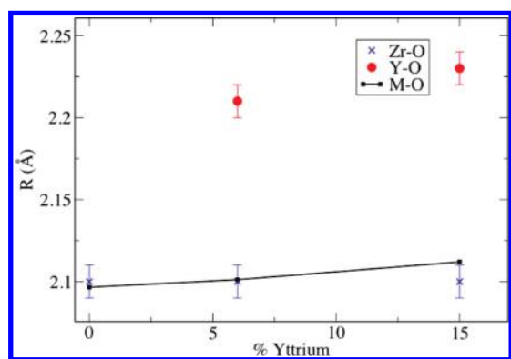
Figure 10. Comparison of first shell Zr-O, Y-O, and M-O distances probed by XRD and EXAFS as a function of Y^{3+} content in hydrated BZY samples.
