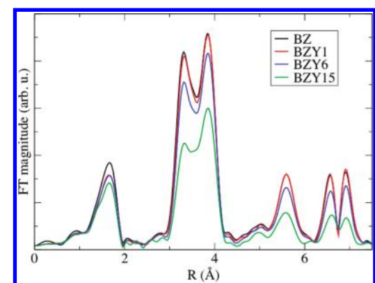
Figure 8. Comparison of Fourier-transformed Zr K-edge EXAFS data of hydrated BZY samples.
