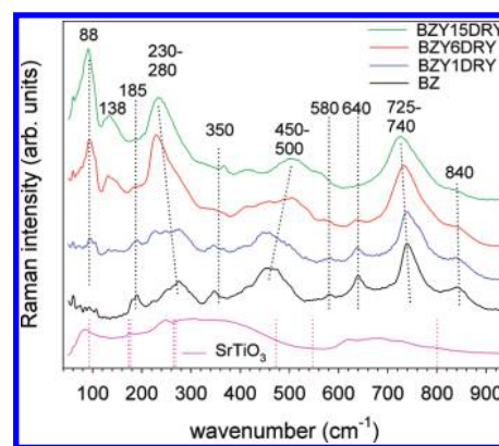
Figure 14. Raman spectra of dry BZY samples with different Y-content, along with the spectrum of undoped SrTiO_3 . Pink dashed lines: phonon modes for cubic SrTiO_3 .
