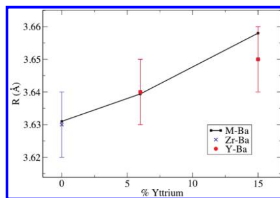
Figure 11. Comparison of second shell Zr-Ba, Y-Ba, and M-Ba distances probed by XRD and EXAFS as a function of Y^{3+} content in hydrated BZY samples. Note that for BZY6 and BZY15, the Zr-Ba symbols and error bars are covered by Y-Ba.
