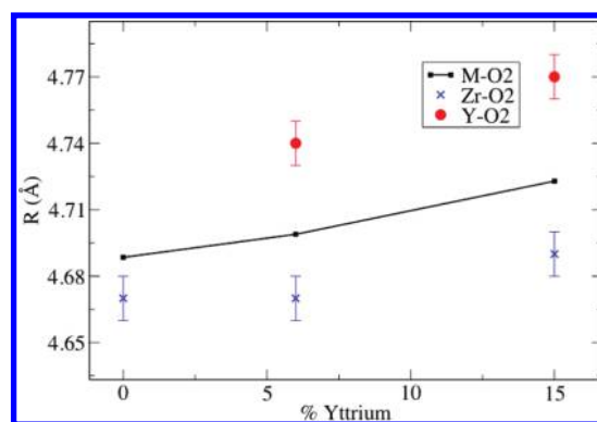
Figure 13. Comparison of fourth shell Zr-O, Y-O, and M-O distances probed by XRD and EXAFS as a function of Y^{3+} content in hydrated BZY samples.
