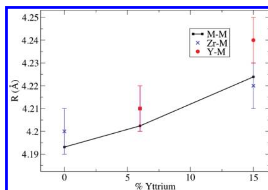
Figure 12. Comparison of third shell Zr-M, Y-M, and M-M distances probed by XRD and EXAFS as a function of Y^{3+} content in hydrated BZY samples. Note that for BZY6, the Zr-M symbol and error bars are covered by Y-M.
