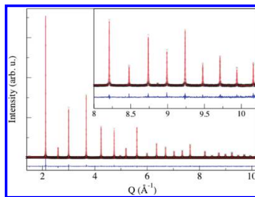
Figure 2. XRD data and model for undoped BZ.
