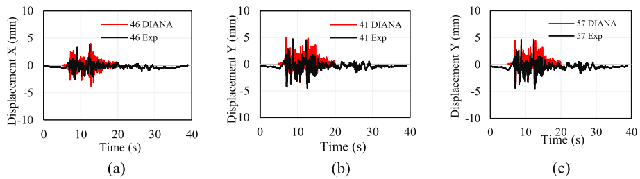
Fig. 24 Comparison of the experimental and numerical displacement histories of selected nodes at Unit 2, for Run 1.3: a Node 46; b Node 41; c Node 57
