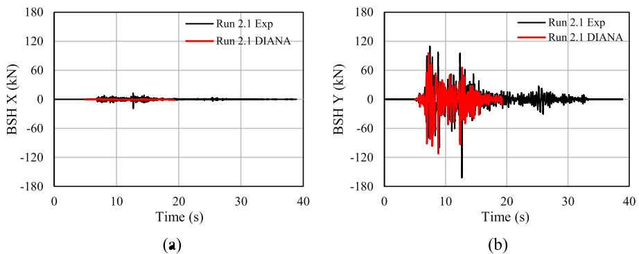
Fig. 28 Comparison of the experimental and numerical base shear force–time histories: (a) Run 2.1X; (b) Run 2.1Y
