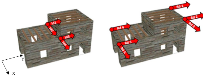
Fig. 6 Displacements relative to the ground (Rd1-6) and interface openings (Id1-4)
