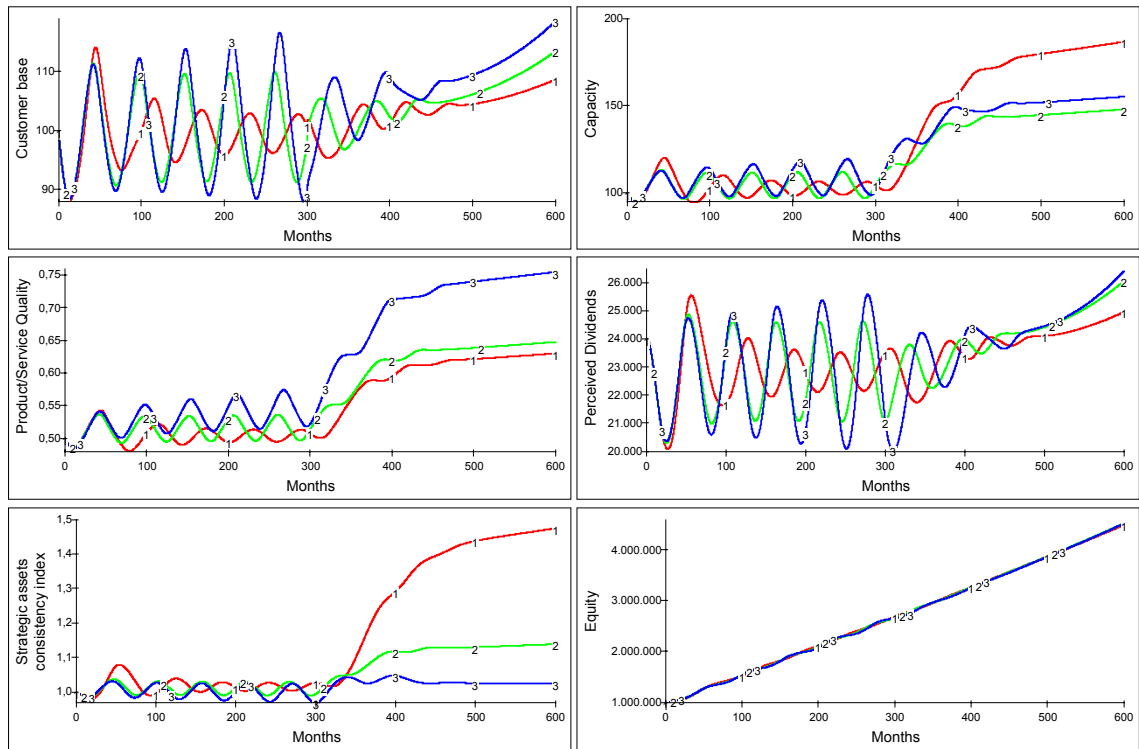
Figure 8 Scenario 5 Behaviours
