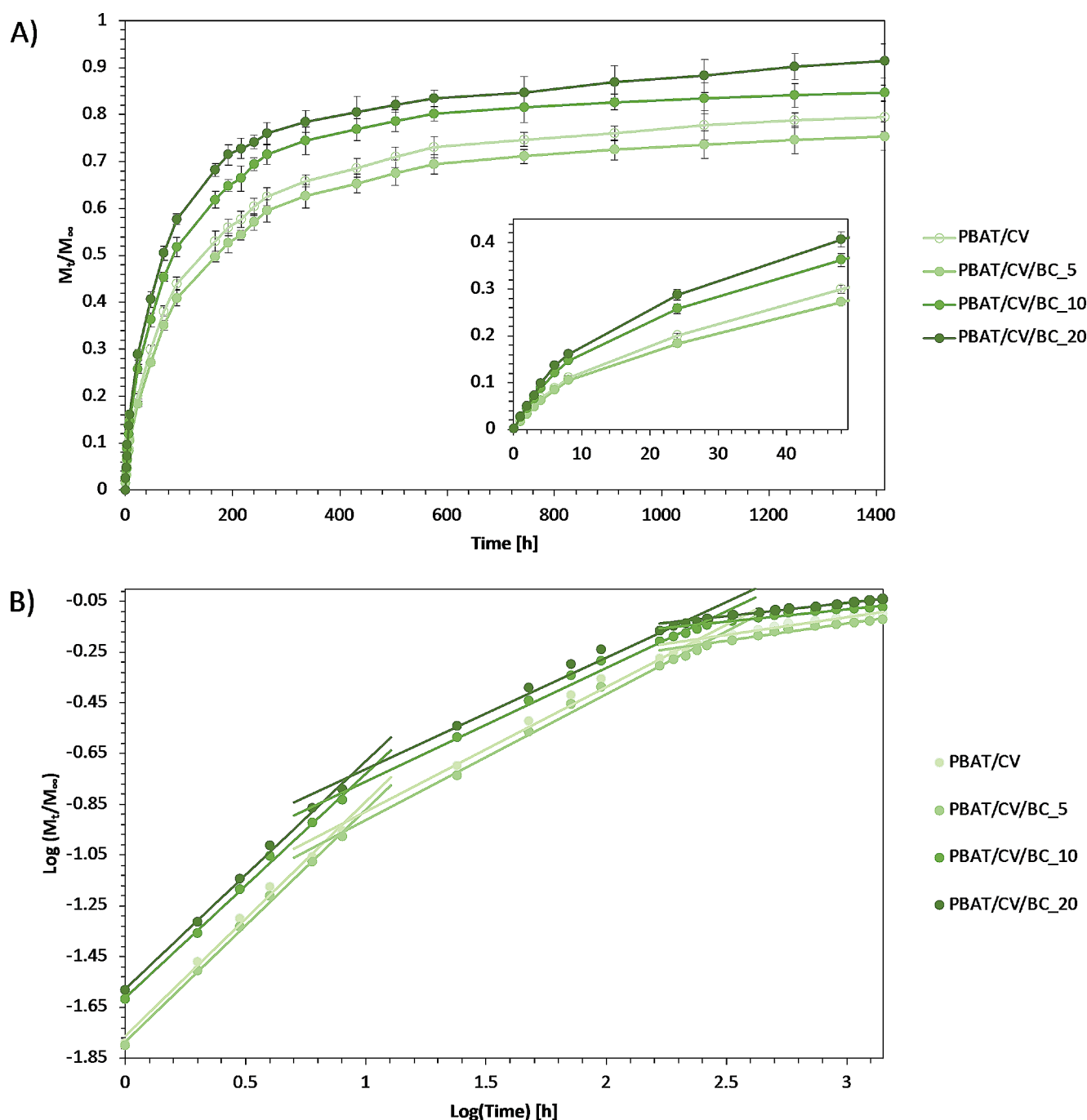
Fig. 10 Release kinetics of CV from PBAT-based films in distilled water at 4 °C expressed as (A) M_t/M_\infty vs. Time and (B) \text{Log}(M_t/M_\infty) vs. \text{Log}(\text{Time})
