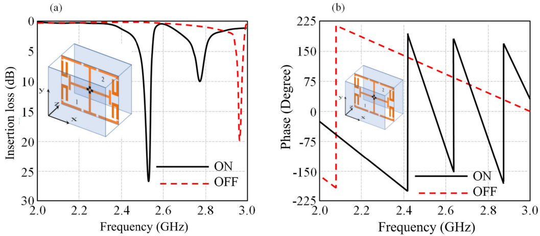
FIGURE 4. Unit cell performance characterization, (a) S_{21} magnitude spectra, and (c) S_{21} phase response.
