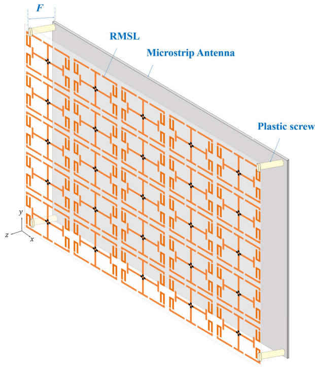
FIGURE 7. The proposed RMSL structure.
