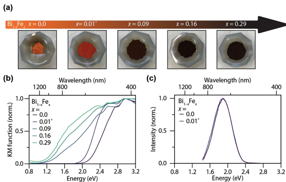
Figure 2. Optical properties of \text{Cs}_2\text{AgBi}_{1-x}\text{Fe}_x\text{Br}_6 . a) Incorporation of \text{Fe}^{3+} into CABB strongly red-shifts the absorption of visible light. b) Kubelka–Munk transform of the diffuse reflectance spectra recorded on the \text{Cs}_2\text{AgBi}_{1-x}\text{Fe}_x\text{Br}_6 samples with ( x = 0.0, 0.01, 0.09, 0.16 , and 0.29 ), showing a gradual red-shift of the absorption onset with increasing \text{Fe}^{3+} -content. The jump in the data \approx 1.4 eV is an artifact of the equipment. c) Photoluminescence spectra of \text{Cs}_2\text{AgBiBr}_6 and \text{Cs}_2\text{AgBi}_{0.99}\text{Fe}_{0.01}\text{Br}_6 . Further increasing the \text{Fe}^{3+} -content quenches the PL almost completely (Figure S5, Supporting Information). *For x = 0.01 the concentration of \text{Fe}^{3+} was below the detection limit of the SEM-EDX.
