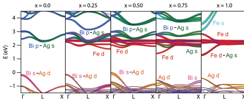
Figure 4. PBE0+SOC bandstructures of \text{Cs}_2\text{AgBi}_{1-x}\text{Fe}_x\text{Br}_6 ( x = 0, 0.25, 0.50, 0.75 , and 1 ). Orbital contributions are indicated in color, omitting contributions of Br p for clarity. All band structures are aligned with respect to a low energy Cs-s state calculated at the \Gamma point. Note that all band structures are calculated within a conventional unit cell setting and assuming ferromagnetic spin ordering (see Supporting Information for a detailed discussion). Due to band folding, the VBM of CABB ( x = 0 ) therefore appears at \Gamma .
