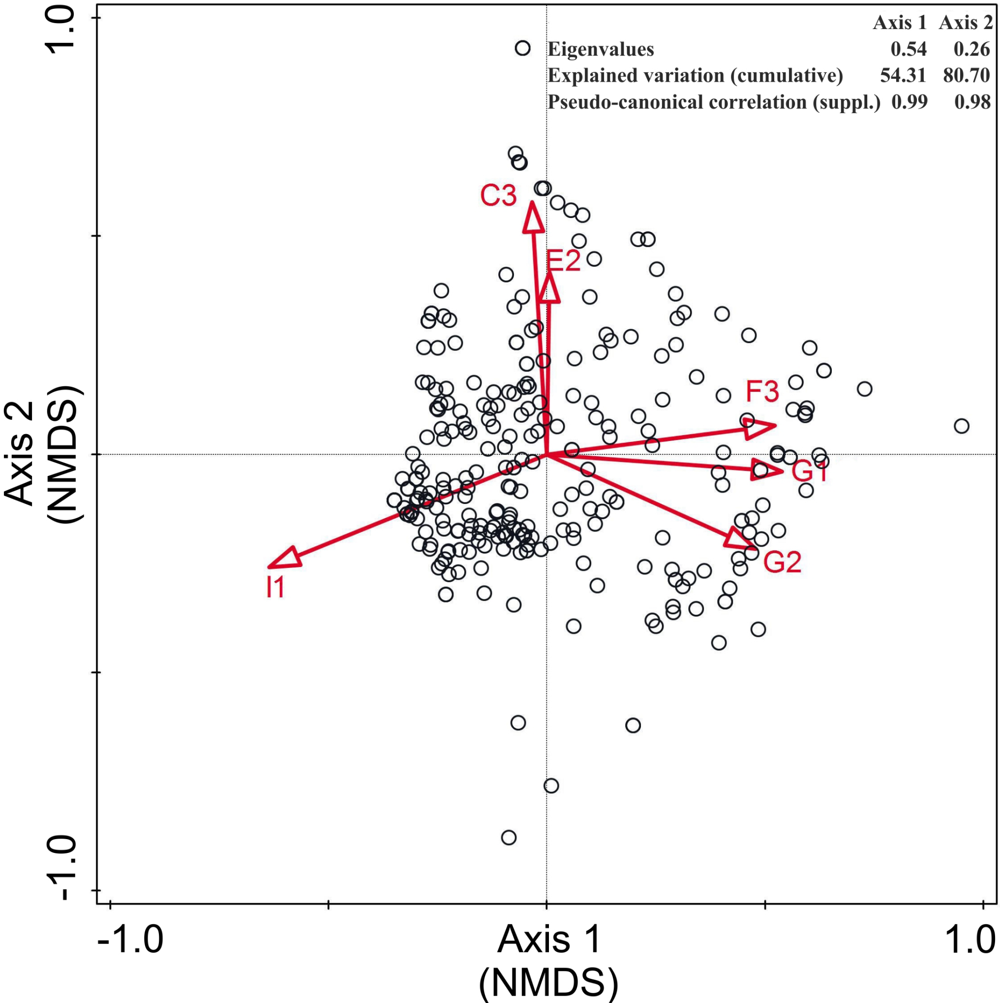
Supplementary Figure S1 | NMDS ordination plot of the NWFP of Sicily with respect to the EUNIS habitats. Only the habitats explaining >3% of the total variance are displayed. C3 = Littoral zone of inland surface water bodies; E2 = Mesic grasslands; F3 = Temperate and Mediterranean montane scrub; G1 = Broadleaved deciduous woodland; G2 = Broadleaved evergreen woodland; and I1 = Arable land and market gardens.
