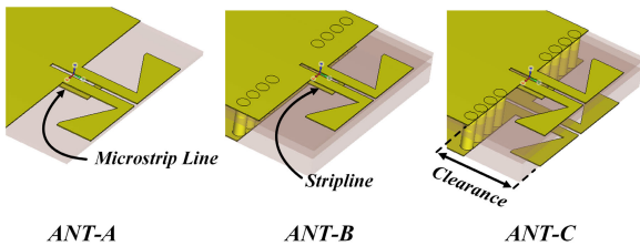
FIGURE 2. Steps evolution of the antenna design process.
