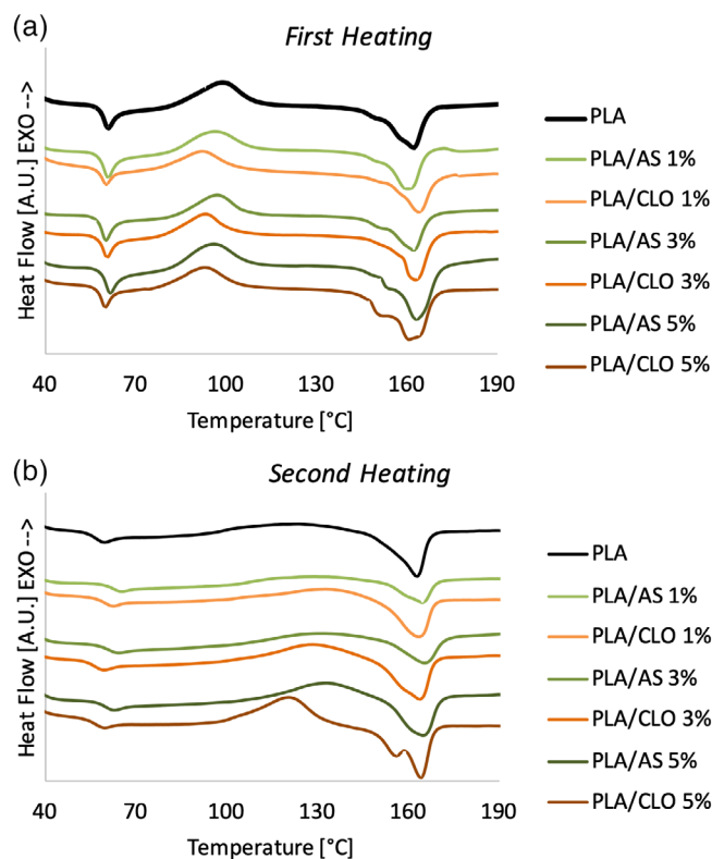
FIGURE 8 Differential scanning calorimetry (DSC) thermograms recorded during (a) first heating and (b) second heating of neat polylactic acid (PLA) and composites
