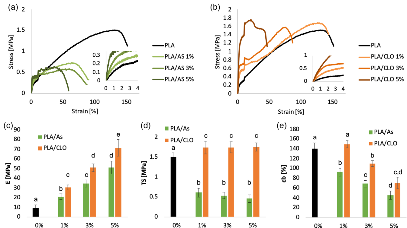
FIGURE 9 Representative stress–strain curves of (a) polylactic acid/silica (PLA/AS) and (b) PLA/clay (CLO) nanocomposites electrospun mats; (c) elastic modulus, (d) tensile strength and (e) elongation at break of PLA/AS PLA/CLO nanocomposites electrospun mats as a function of the filler content. Values are given as means ± SD of n = 5 samples. Different letters in the same graph indicate significant differences ( p < .05 ) when analyzed by multiple Student's t test
