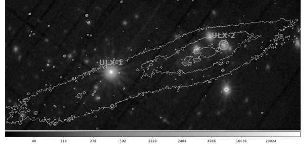
Figure 1. XMM-Newton stacked image of NGC 55. Circles with 20'' radii are drawn around the ULXs along with surface brightness contours from the filter-RG610 DSS image. The color bar shows the number of counts.
