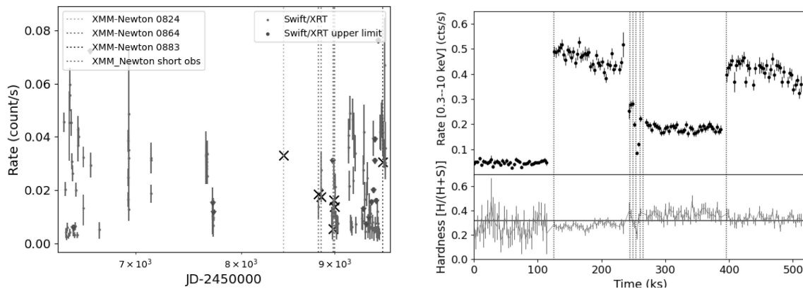
Figure 3. Left: 0.3–10 keV long-term Swift /XRT light curve of NGC 55 ULX-2, with the dates of the XMM-Newton observations indicated by vertical dotted lines and the equivalent XRT count rates indicated by black ‘X’. Right: 0.3–10 keV XMM-Newton / EPIC-pn light curve of NGC 55 ULX-2. Since the observations occur at different epochs, we removed the gaps between observations with grey-dashed lines for displaying purposes.
