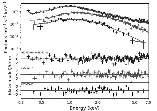
Figure 2. XMM-Newton spectra of NGC 55 ULX-2 candidate. For visual purposes, only EPIC-pn data are shown. The best-fit DBB+COMT model is overlapped (red, solid line). The bottom panels show the corresponding residuals.
