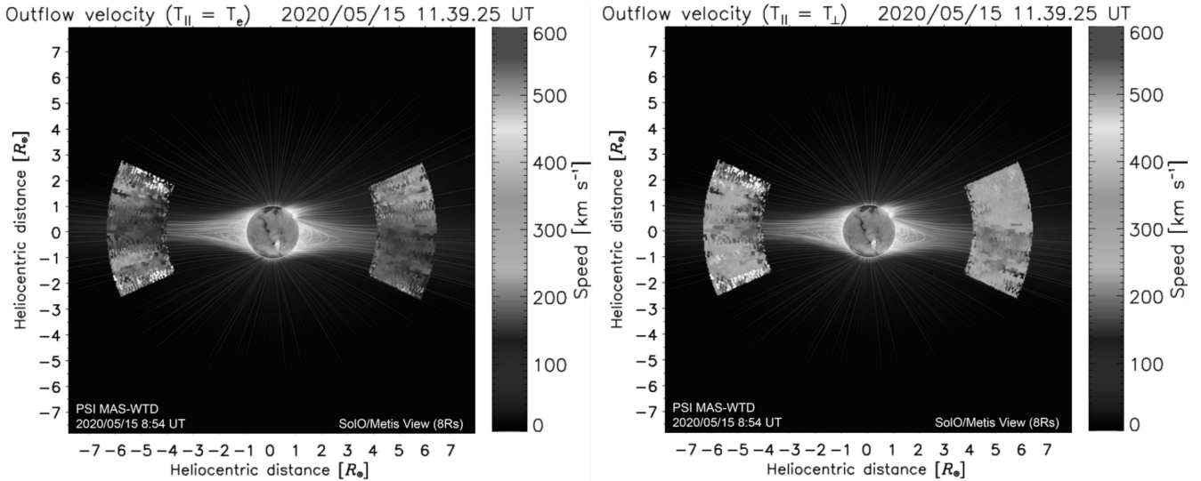
Fig. 4. HI outflow velocity map, within the region where the S/N is equal to 5, in the case of anisotropy, T_{\text{HI},\parallel} = T_e (left panel) and of isotropy T_{\text{HI},\parallel} = T_{\text{HI},\perp} (right panel) of the neutral hydrogen kinetic temperature along the radial direction.
