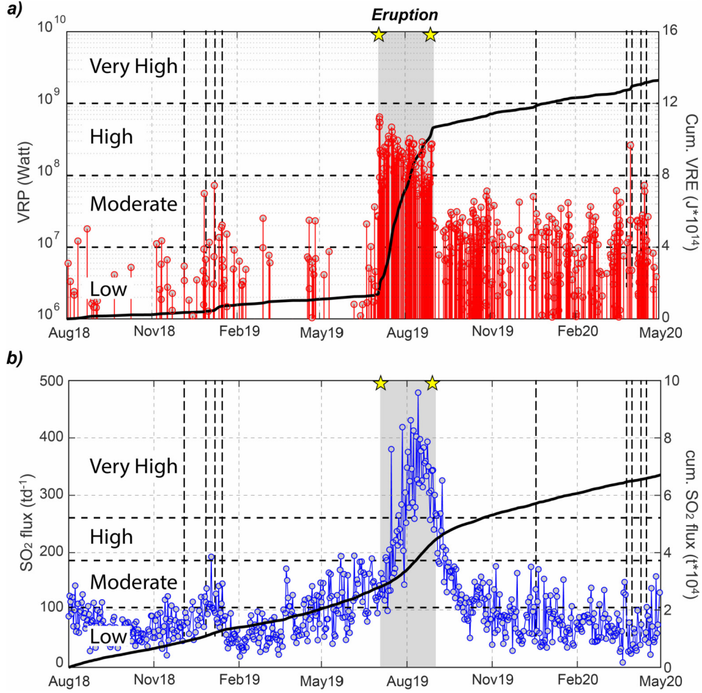
Fig. 2. (a) Volcanic Radiative Power (VRP), in logarithmic scale, and (b) \text{SO}_2 flux, in linear scale, from August 2018 to May 2020 in relation with the activity thresholds, retrieved by ten-years and five-years long databases, as represented by the horizontal dotted lines (Coppola et al., 2016; LGS Report), together with their associated cumulative thermal energy (Volcanic Radiant Energy; VRE in Joule) and \text{SO}_2 masses emitted (in tons). Yellow stars indicate the two paroxysmal explosions; grey field represents the effusive period and the dashed lines marked episodic overflows and/or spattering activity as reported by periodic bulletin (see text for details). (For interpretation of the colors in the figure(s), the reader is referred to the web version of this article.)
