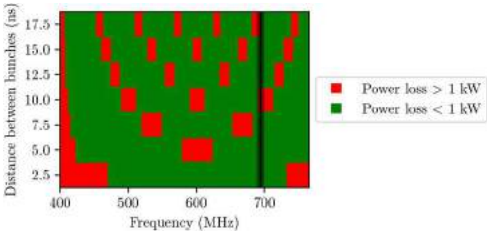
Fig. 3.23. Calculated power loss map for a single-cell cavity. Frequency ranges with acceptable power losses below 1 \text{ kW} for different bunch spacing are shown in green. Regions with power losses above 1 \text{ kW} are shown in red. The dark vertical line corresponds to the position of a HOM of the single-cell cavity design with the maximum frequency shift of 5 \text{ MHz} . The bunch spacings of 10 \text{ ns} and 17.5 \text{ ns} are not acceptable for this HOM due to high power losses (see, overlap of red with black regions). The frequency range for the calculations is limited by the fundamental mode frequency ( 400.79 \text{ MHz} ) and the cut-off frequency ( 765 \text{ MHz} ).
