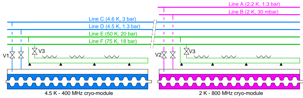
Fig. 5.14. Cryogenic flow scheme of FCC-ee CMs (here the cryogenic plant is located to the right of the 800 MHz section).
