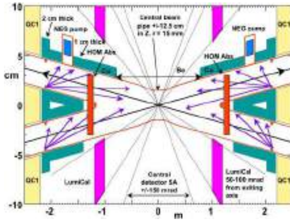
Fig. 2.18. x - z view of the FCC-ee interaction region layout for \pm 2.5 m from the interaction point. Note the different horizontal (m) and vertical (cm) scales.
