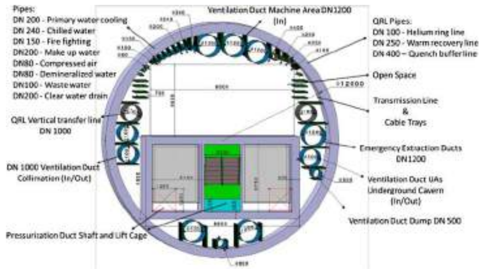
Fig. 4.6. Service shaft cross-section.
