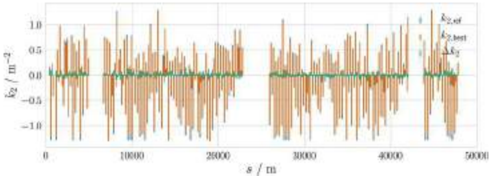
Fig. 2.16. Change in sextupole strengths (green) between optimised solution (red) and reference solution (blue) for one half ring.
