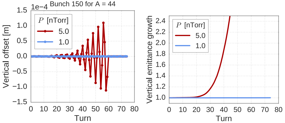
Fig. 2.37. Bunch train evolution over 75 turns for CO 2 ( A = 44 ) gas in the arcs, with 7.5 ns bunch spacing: vertical centroid motion of the last bunch (left) and vertical emittance growth of most unstable bunch (right).
