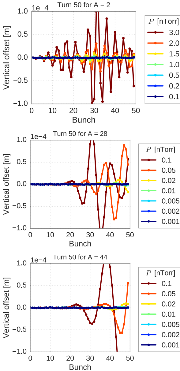
Fig. 2.36. Vertical bunch centroid offsets after 50 turns with selected pressures of H 2 , CO and CO 2 gas (from top to bottom) in the straight section model with 2.5 ns bunch spacing.
