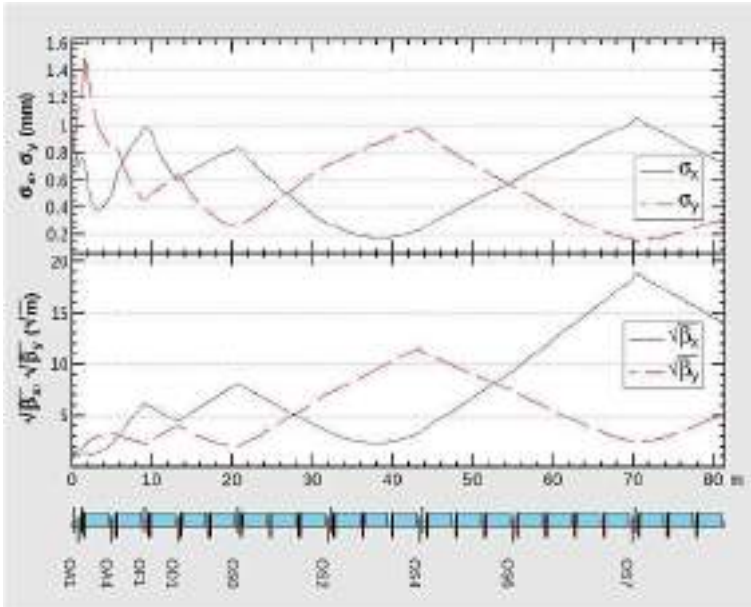
Fig. 6.4. Optics of the 1.54 GeV linac.
