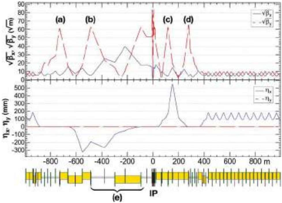
Fig. 2.7. The beam optics of the FCC-ee IR for t\bar{t} . Upper and lower rows show \sqrt{\beta_{x,y}} and dispersions, respectively. The beam passes from the left to the right. The optics is asymmetric to suppress the synchrotron radiation toward the IP. Dipoles are indicated by yellow boxes; those in region (e) have a critical energy of the SR photon below 100 keV at the t\bar{t} . Sextupoles for the LCCS are located at (a–d), and sextupoles at (a,d) play the role of crab sextupoles.
