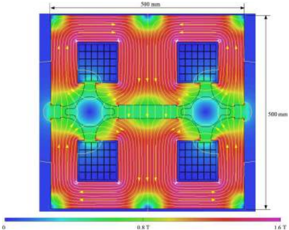
Fig. 3.3. Cross-section of the FCC-ee main quadrupole, for a 10 T/m gradient.
