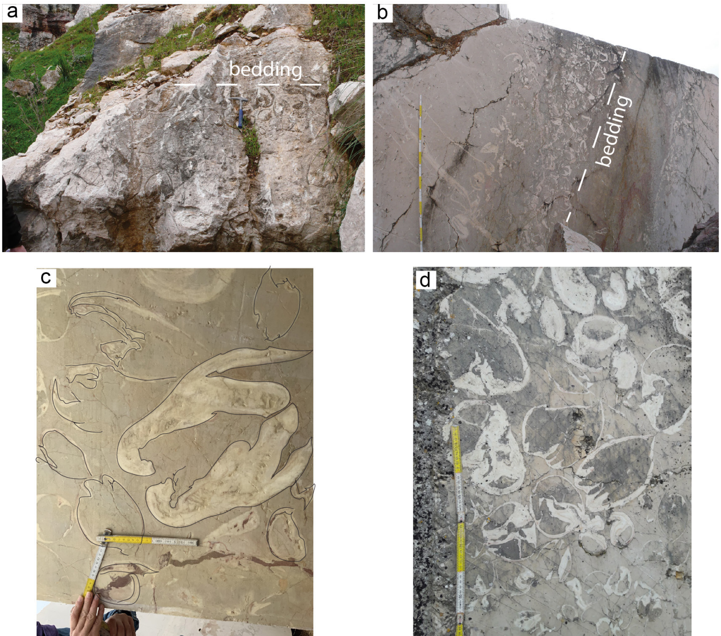
Fig. 4 - Megalodontoids assemblages (highlighted by a black line) from Unit A: a) large megalodontoids in growth position; b) a subtidal facies showing predominant disarticulate valves of megalodontoids; c) a quarried block showing large Dicerocardium spp.; d) an assemblage of large Neomegalodon sp. notice that also small specimens are present in the lower part of the image.
