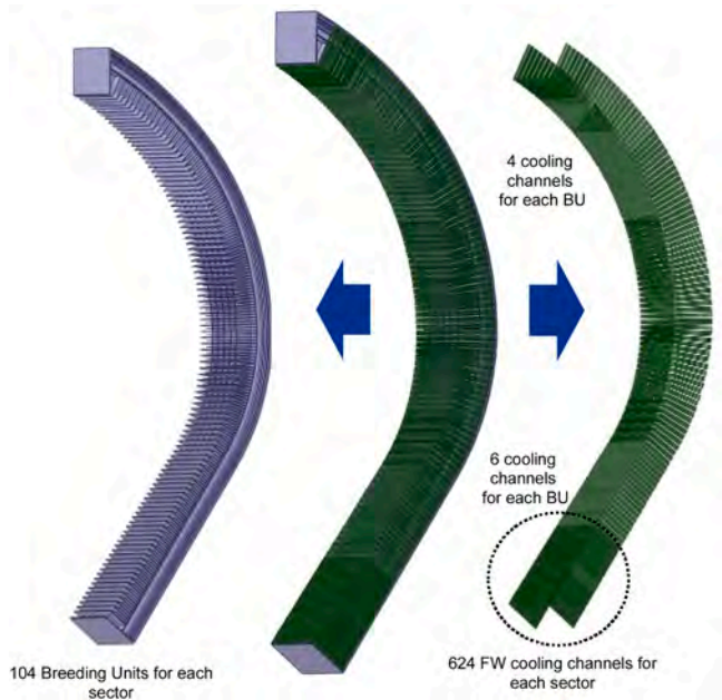
Fig. 6. WCLL DEMO outboard sector structure: BU layout (left) and poloidal distribution of the FW cooling channels (right).
