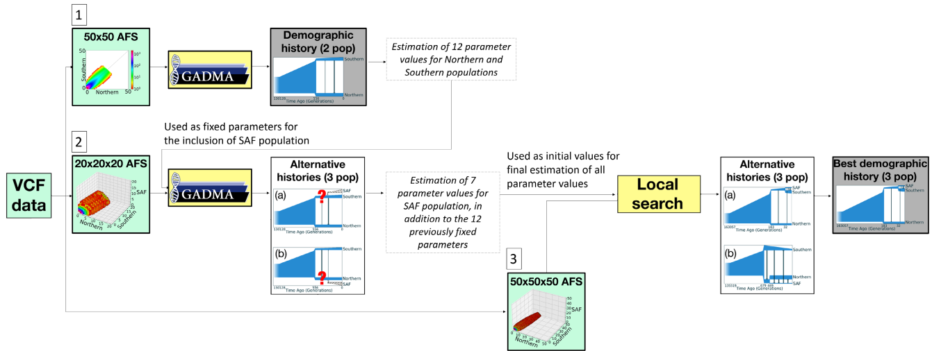
FIGURE 3 A scheme of demographic inference for two and three populations of the blue shark, Prionace glauca . The 2-population model (upper part, [1]) distinguished northern (Atlantic Ocean and Mediterranean Sea) from southern (Indian and southwestern Pacific oceans) populations. The 3-population models (middle and lower part, [2] and [3]) distinguished south African, northern (Atlantic Ocean and Mediterranean Sea) and southern (Indian and southwestern Pacific oceans) populations, with the two tree models differing depending on the late divergence of SAF from the northern (a) or southern (b) group. Light green colour corresponds to the data used (size and dimensions of the observed JAFS, obtained from DATA 4 converted into a VCF file). Light yellow refers to the algorithms used. White and grey refer to the evaluated scenarios, the latter representing the scenario identified as the most likely to explain the observed genetic variation.
