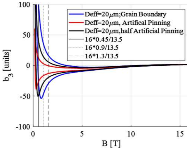
Fig. 3. Sextupolar field error b_3 of the 16 T dipole magnets, in units of 10^{-4} at a reference radius of 16.7 mm, as a function of field strength, for an effective Nb 3 Sn filament size of 20 \mu\text{m} , without flux pinning (blue), with 100% artificial pinning (red), and with a realistic 50% pinning efficiency (black). Three different injection energies are indicated.
