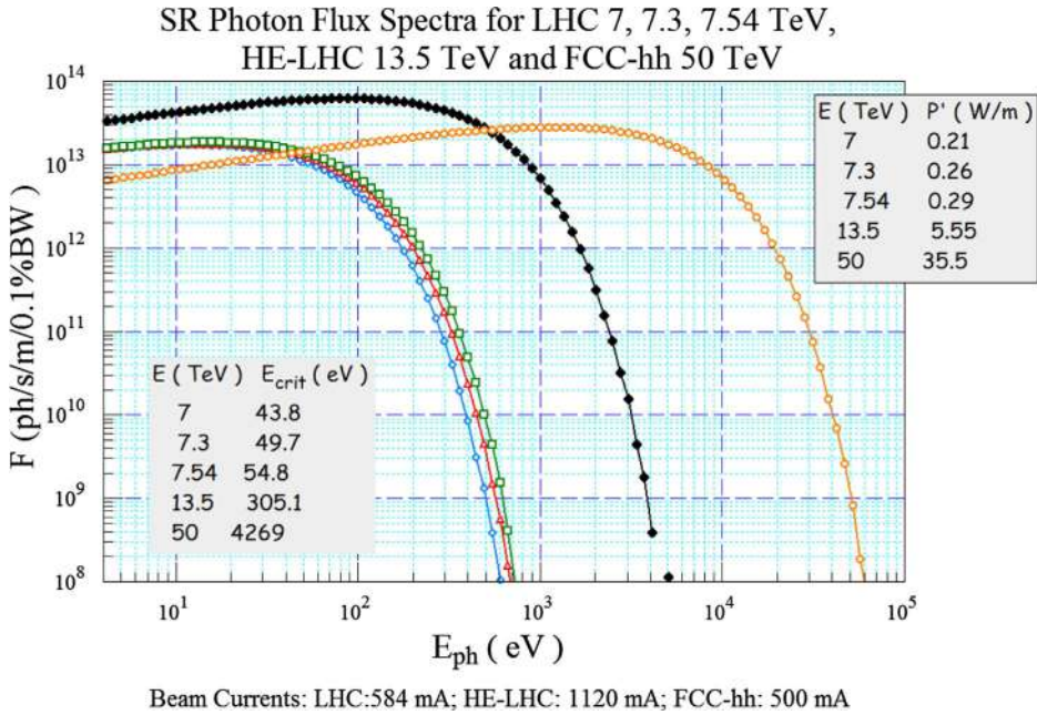
Fig. 3.9. Comparison of the SR flux spectra for LHC at three energies, HE-LHC and FCC-hh.
