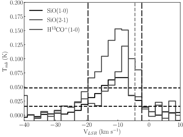
Figure 4. SiO(1-0) (black), SiO(2-1) (red), and \text{H}^{13}\text{CO}^+ (1-0) (green) spectra extracted towards the regions of the map with emission above the 3\sigma levels. The horizontal dashed lines indicate the 3 \times \text{rms} levels for each species. Vertical blue dash-dotted lines indicated the velocity range considered for the comparison with RADEX models. Finally, the vertical grey line indicates the central velocity of IC443.
