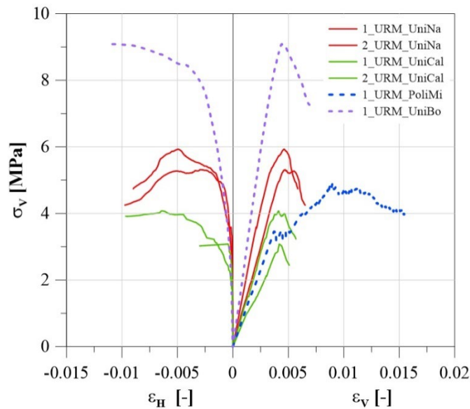
Fig. 18. Axial stress vs. axial and hoop strain for unreinforced clay brick masonry specimens.
