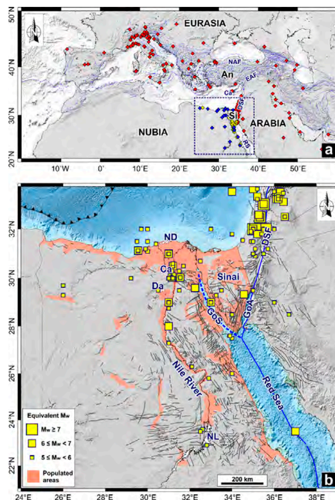
Figure 1. (a) Map of the Mediterranean region showing the main tectonic plates. Active faults are reported as blue lines. The GNSS (Global Navigation Satellite System) stations analyzed in this study are reported as blue (EPGN—Egyptian Permanent GPS Network), red (EUREF [8], SOPAC [9] and UNAVCO [10]) and yellow (survey-type) diamonds. The dashed blue box represents the Scheme 11 (study region). Abbreviations are: Si, Sinai plate; An, Anatolian plate; NAF, North Anatolian fault zone; EAF, East Anatolian fault zone; Ca, Cyprian Arc system; DSF, Dead Sea fault system; RS, Red Sea basin; (b) Simplified tectonic map of Egypt and its surrounding areas. Thin black lines denote major surface faults [11]; thick blue lines stand for plate boundaries [5]. Populated areas [12] and historical seismicity (spanning the 2200 B.C.–1899 A.D. period [13]) are also reported. Abbreviations are: ND, Nile Delta; Ca, Cairo; GoS, Gulf of Suez; GoA, Gulf of Aqaba; Da, Dahshour; NL, Nasser’s Lake.
