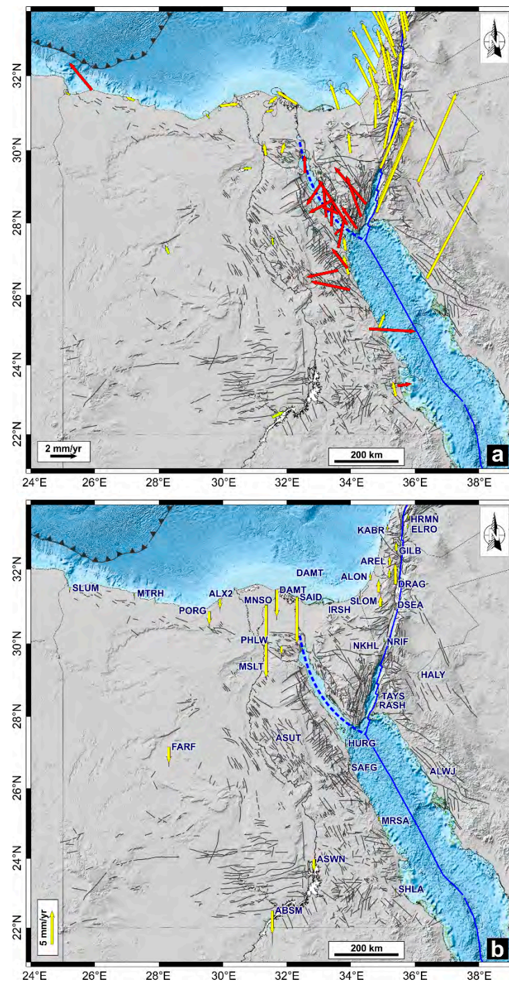
Figure 4. (a) Horizontal GNSS velocities and 95% confidence ellipses in a fixed Eurasian plate (see Table S2 for details). Continuous and episodic GNSS stations are reported as yellow and red arrows, respectively; (b) vertical GNSS velocities and 95% confidence uncertainties.
