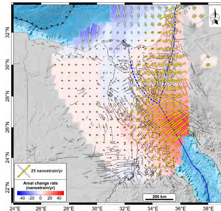
Figure 5. Geodetic strain-rate parameters: colors range in the background shows the magnitude of the areal change rate, while arrows represent \epsilon_{Hmax} (yellow) and \epsilon_{hmin} (white) horizontal strain-rate axes.
