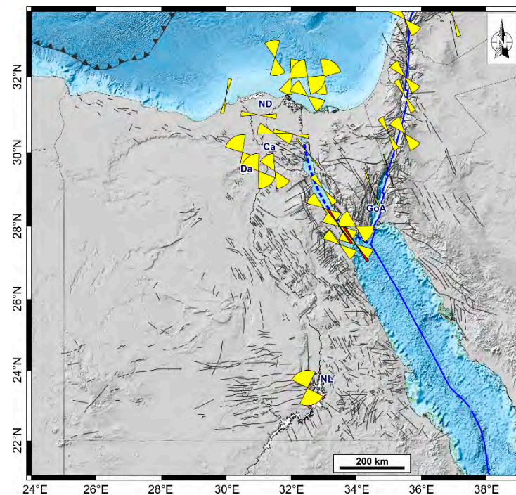
Figure 7. Rotational wedges illustrating the angular difference between the averaged azimuths of the axis of maximum horizontal compressive stress ( S_{Hmax} ) and the axis of the minimum strain-rate \epsilon_{hmin} over the investigated region. The two rotational wedges reported in red, for the southern sector of the Gulf of Suez, show the angular difference between the S_{Hmax} estimated by only seismic data (Table 1) and the \epsilon_{hmin} axis. Abbreviations are: ND, Nile Delta; Ca, Cairo; Da, Dahshour; NL, Nasser's Lake; GoA, Gulf of Aqaba.
