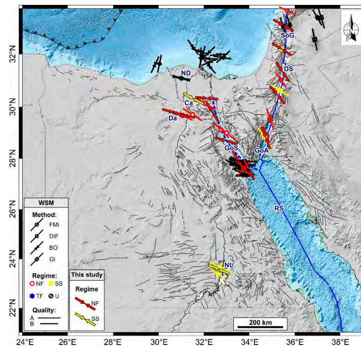
Figure 6. Map of the present-day stress field (in terms of S_{Hmax} orientation) inferred from FPSs inversions (FMI), drilling-induced fractures (DIF), borehole breakouts (BO) and geological indicators (GI). NF, normal faulting; SS, strike-slip faulting; TF; thrust faulting; U, undefined. “A” and “B” are quality ranking as defined in [80]. Results achieved in this study are reported as large arrows and colored according to the inferred stress regime (Table 1). Abbreviations are: ND, Nile Delta; Ca, Cairo; Da, Dahshour; NL, Nasser’s Lake; SoG, Sea of Galilee; DS, Dead Sea; GoA, Gulf of Aqaba; GoS, Gulf of Suez; RS, Red Sea.
