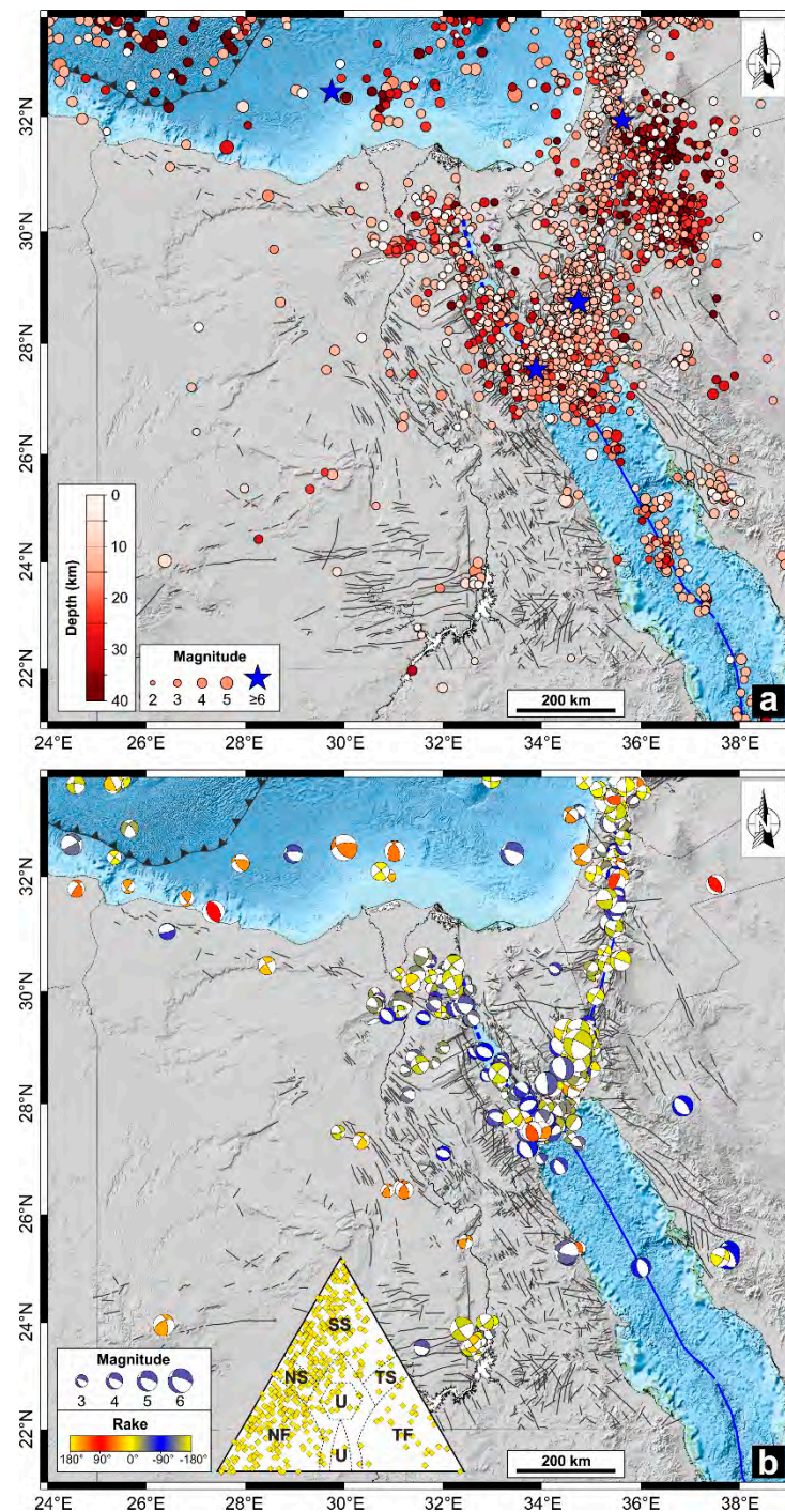
Figure 2. (a) Instrumental crustal seismicity (1927–2020) of Egypt, collected from the International Seismological Center bulletin [34]; (b) lower hemisphere, equal area projection for the 451 fault plane solutions (FPSs) compiled for this study. FPSs are colored according to the value of the rake angle: red, blue and yellow indicate pure thrust faulting, pure normal faulting and strike-slip faulting, respectively. A ternary plot of FPSs is also reported: each point is plotted based on the plunge of the P, T, and B axes of the FPSs [35]. The dashed lines divide the diagram into faulting styles [14]: NF is normal faulting, NS is normal and with strike-slip component, SS is strike-slip faulting, TS is thrust with strike-slip component, TF is thrust faulting, and U is undefined.
