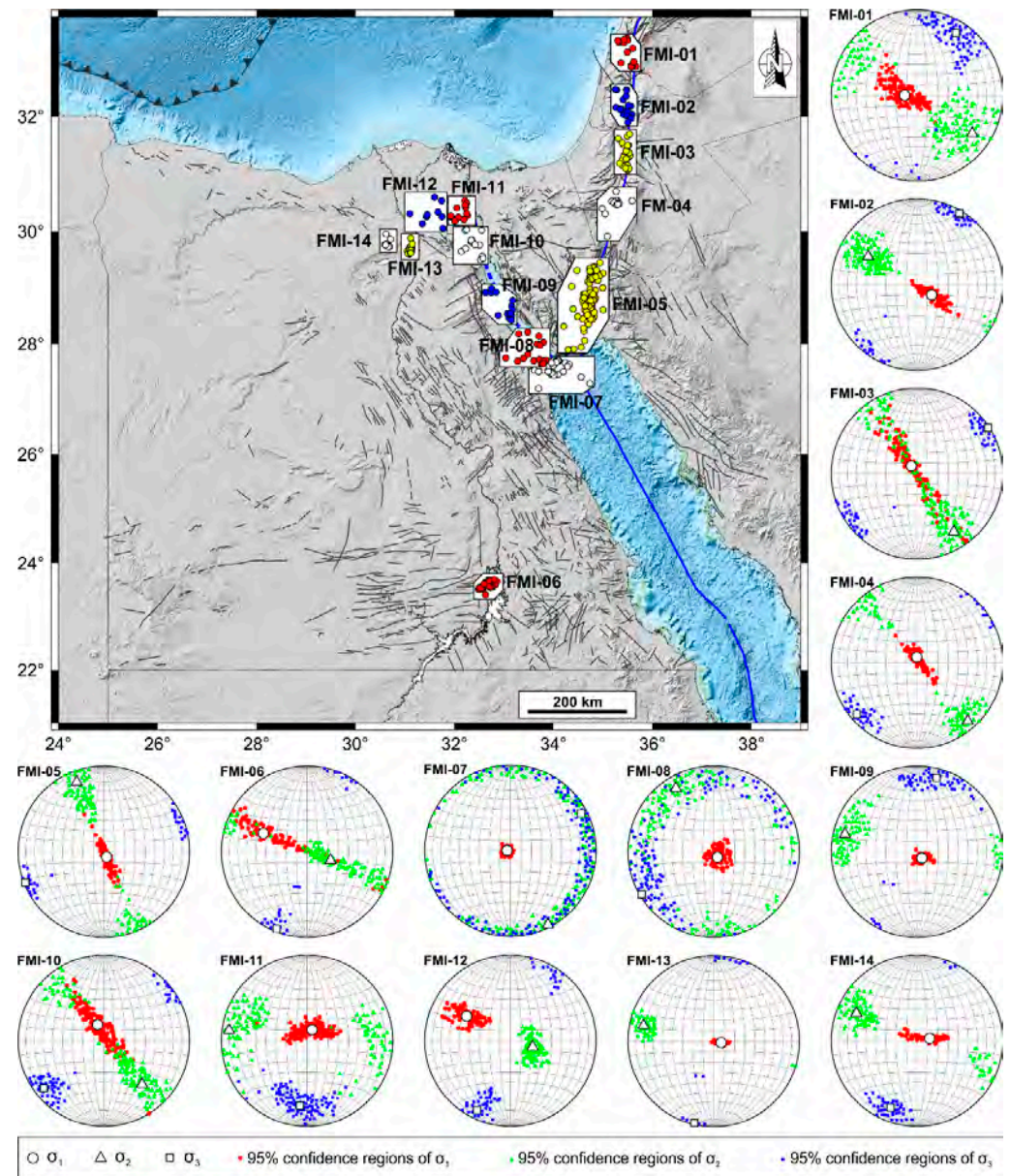
Figure 3. The map shows the 14 subsets selected for the stress tensor inversion. The principal stress axes with their 95% confidence regions are also plotted on lower hemisphere stereonets (see Table 1 for details).
