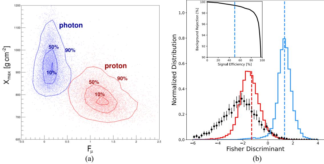
FIG. 6. (a) X_{\max} - F_{\mu} distributions for photons (blue) and protons (red). Contour lines enclose the 90%, 50%, and 10% of the distributions of the events, reweighted to a realistic power law spectrum E^{-\Gamma} ( \Gamma = 2.7 for protons and \Gamma = 2.0 for photons) [35]. (b) Distribution of the Fisher discriminant for simulated photons (signal, blue) and protons (background, red), and for the burnt sample (black). The vertical red line indicates the value of the Fisher discriminant ( f = -1.3 ) above which the background begins to decrease nearly exponentially, while the photon selection efficiency is still very close to 100%; the blue line indicates the median of the photon distribution. Inset: background rejection as a function of signal efficiency obtained with the Fisher discriminant analysis.
