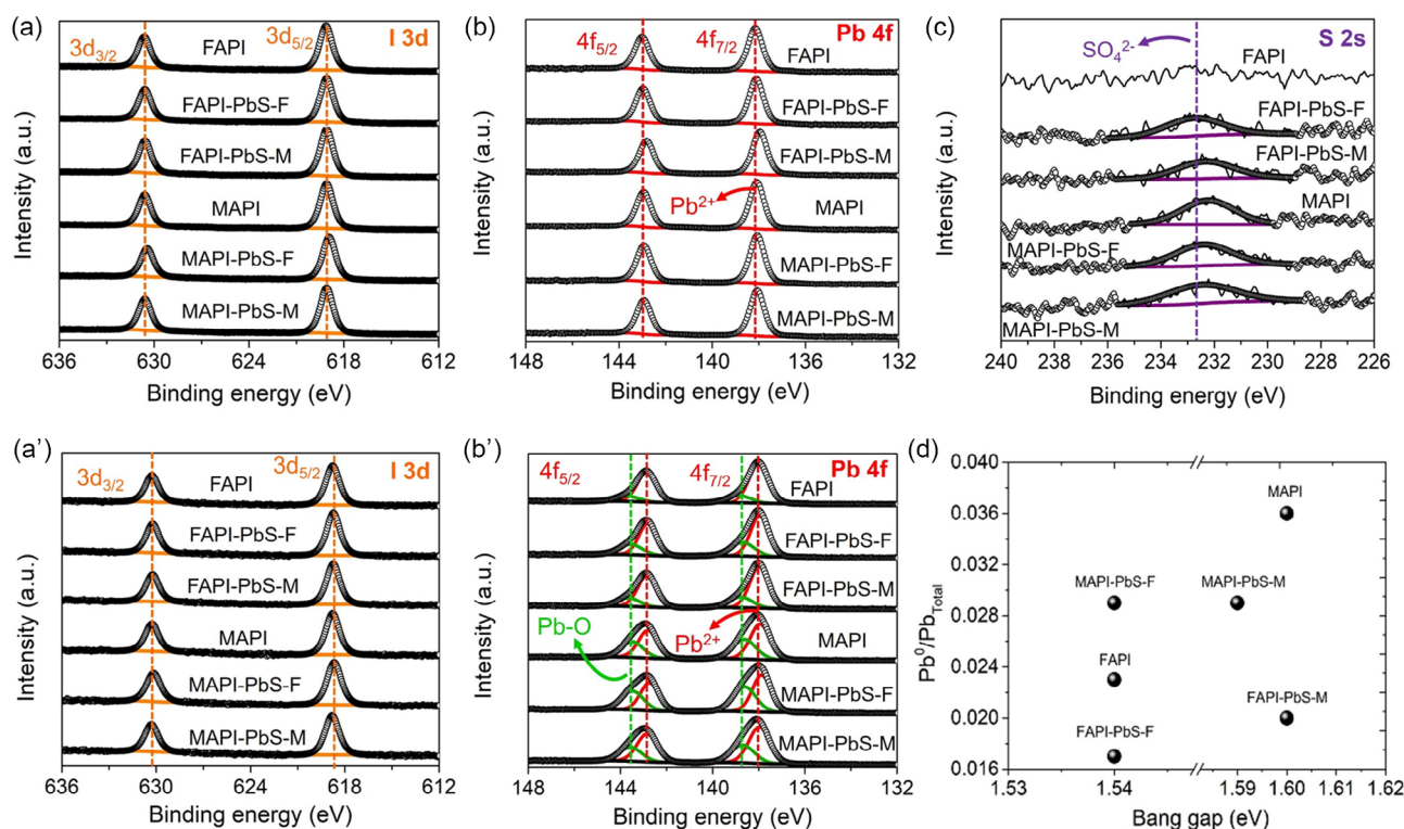
Figure 4. HR-XPS: a,a') I 3d, b,b') Pb 4f, c) S 2s spectra, d) calculated metallic lead-to-total lead (Pb 0 /Pb total ) ratio versus experimentally observed optical bandgap of FAPI, FAPI-PbS-F, MAPI-PbS-F, MAPI, FAPI-PbS-M, and MAPI-PbS-M-based perovskite thin films. (a,b) Before and (a',b', and c) after 30 days under ambient air aging.
