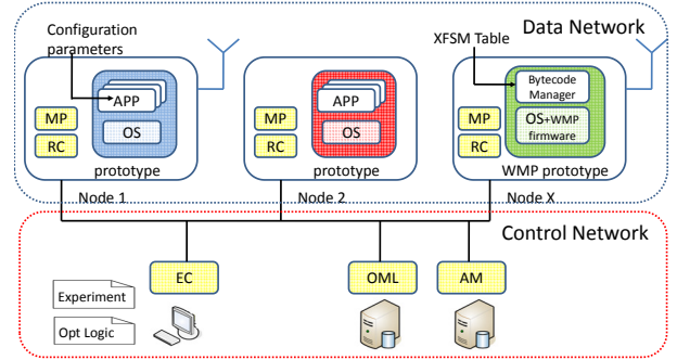
Figure 1: WMP integration in the OMF architecture as a specific node prototype.
