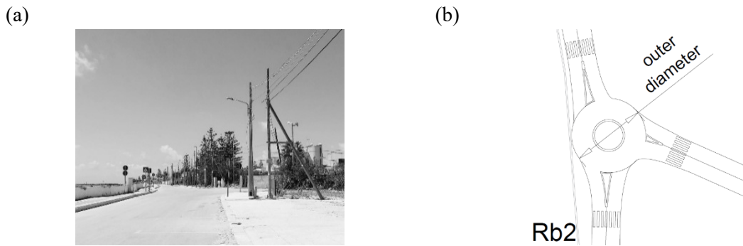
Fig. 5. Intersection view: (a) current intersection area in which Roundabout 2 (Rb2) was designed and (b) the designed three-legged single-lane Roundabout 2 (Rb2)
