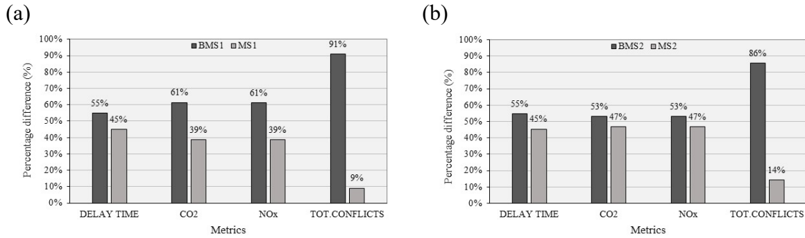
Fig. 8. Percentage ratios of delay time, pollutant emissions, and total conflicts evaluated with respect to their total simulated values considering (a) mobility scenario 1 (MS1) and baseline mobility scenario 1 (BMS1) and (b) mobility scenario 2 (MS2) and baseline mobility scenario 2 (BMS2)
