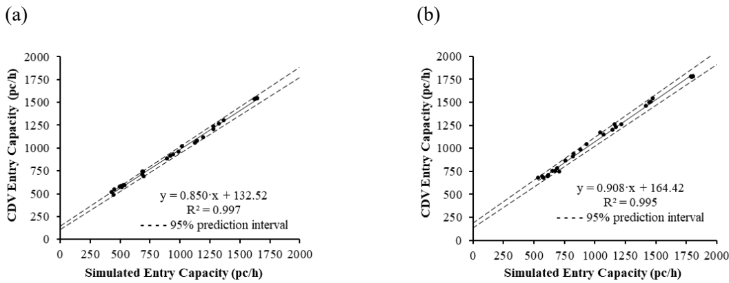
Fig. 7. Scatterplots for (a) mixed traffic with 40% CDVs and 60% HDVs and (b) mixed traffic with 80% CDVs and 20% HDVs
