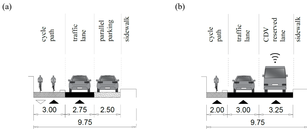
Fig. 3. The roadway cross section: (a) current configuration and (b) designed configuration. All measures are indicated in meters. CDVs = cooperative driving vehicles
