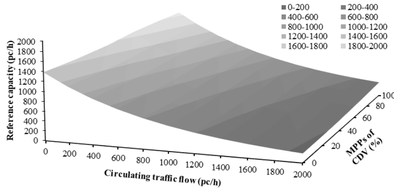
Fig. 6. Surface of reference capacity function
