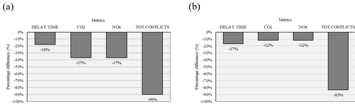
Fig. 9. Percentage difference between the designed solution and the current one, simulating (a) mobility scenario 1 (MS1) and baseline mobility scenario 1 (BMS1) and (b) mobility scenario 2 (MS2) and baseline mobility scenario 2 (BMS2)
