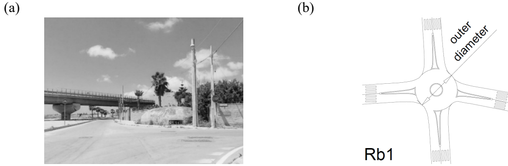
Fig. 4. Intersection view: (a) current area in which Roundabout 1 (Rb1) was designed and (b) the designed four-legged single-lane Roundabout 1 (Rb1)
