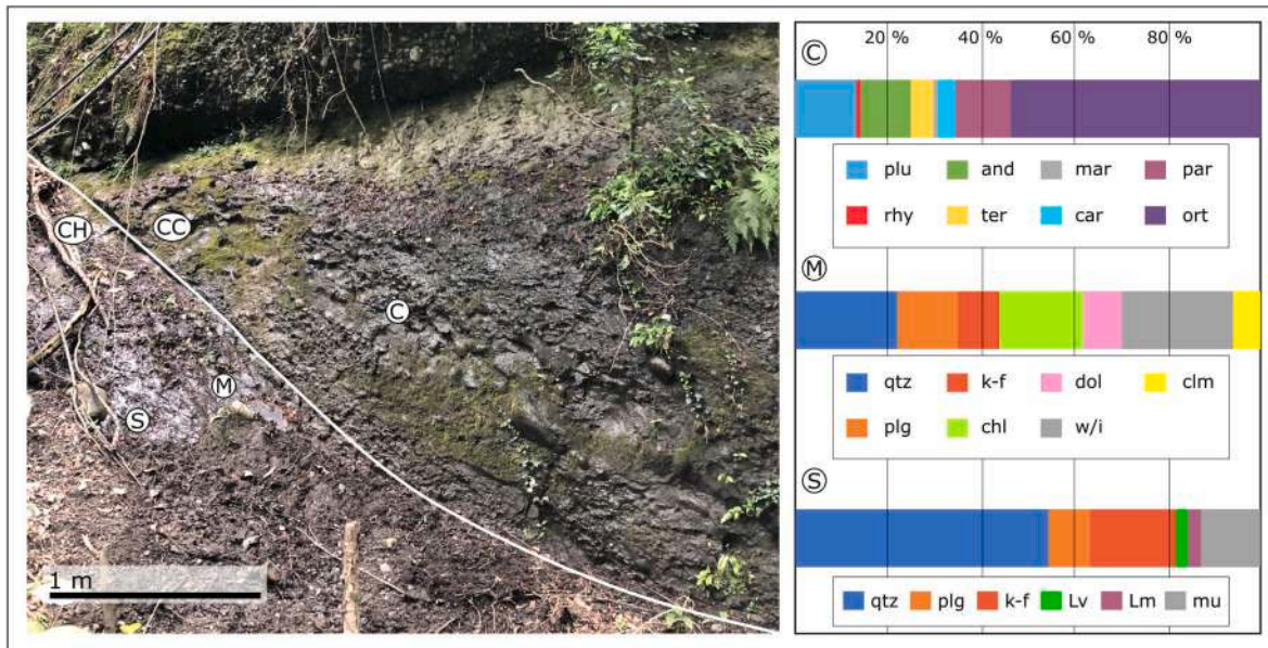
Fig. 7. Comparison among compositions of a sandy (S) layer, point-counted through Gazzi-Dickinson method, a muddy layer (M) through XRD analyses, and a conglomerate bed (C), gain through lithological association of the gravel-sized detritus (from Di Capua et al., 2016a,b) of section MO. Plu: plutonic rocks; And: andesites; mar: marls; par: paragneiss; rhy: rhyolites; ter: terrigenous; car: carbonate rocks; ort: ortogniess; qtz: quartz; k-f: k-feldspar; dol: dolomite; clm: clay minerals; plg: plagioclase; chl: chlorite; w/i: muscovite/illite; Lv: volcanic lithics; Lm: metamorphic lithics; mu: muscovite.
