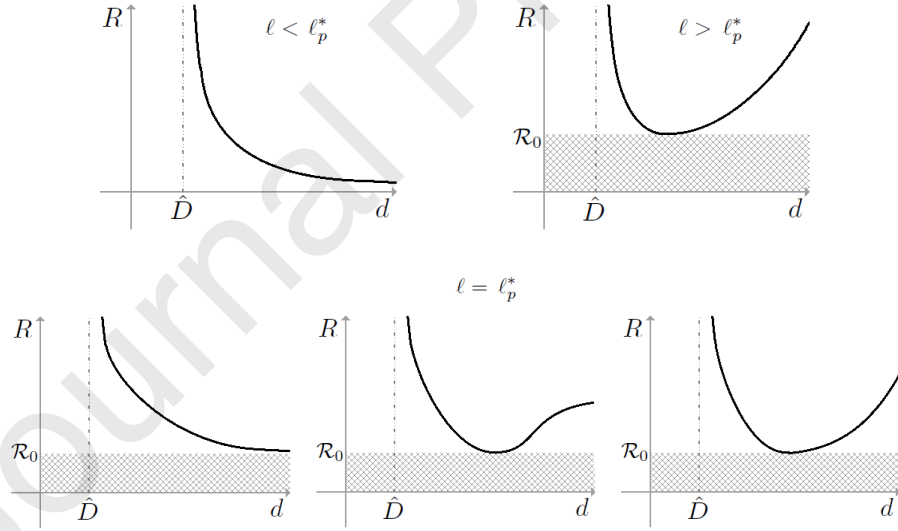
Figure 2: A sketch of the graph of the function R(d) , in the setting of Theorem 3. In the critical case \ell = \ell_p^* , we have three possible alternatives.
