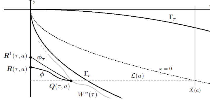
Figure 4: The position of the points Q(\tau, a) , R(\tau, a) , and R^1(\tau, a) .
