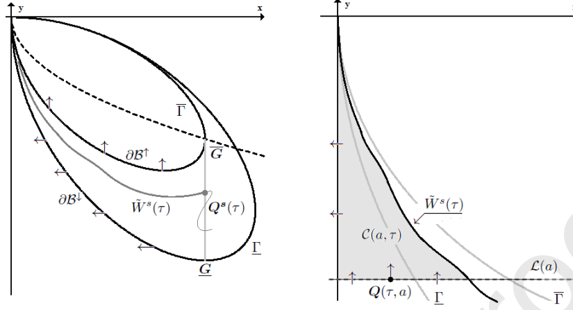
Figure 5: The constructions needed in the proof of Lemma 45.
