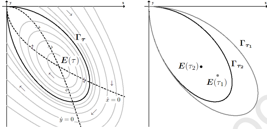
Figure 3: On the left, the energy levels of \mathcal{H} at fixed time \tau , with the homoclinic orbit \Gamma_\tau . On the right, the position of the set \Gamma_{\tau_2} with respect to the set \Gamma_{\tau_1} in the case K(\tau_2) > K(\tau_1) .
