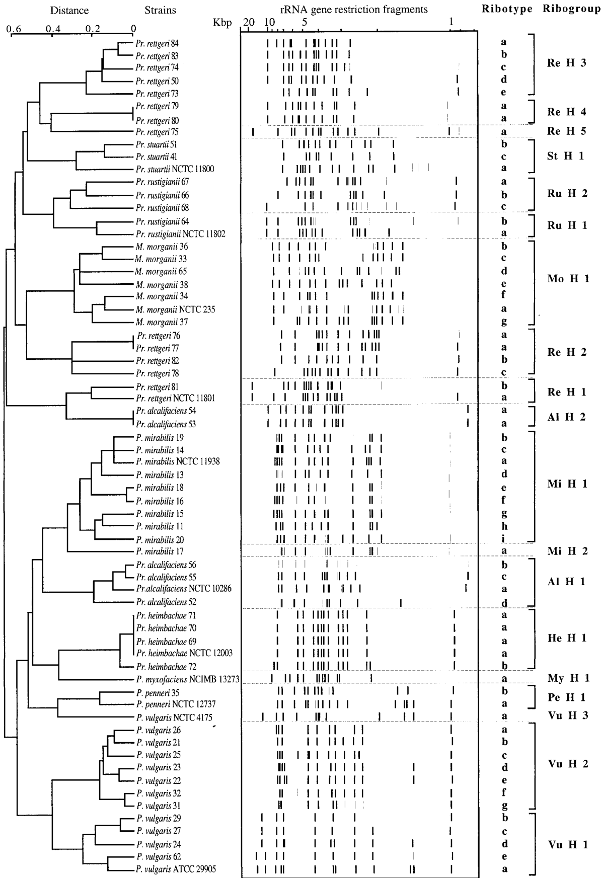
FIG. 6. Dendrogram based on the Hinc II restriction patterns of 66 strains listed in Table 1. The distance matrix was generated by using the complement of Dice similarity coefficients and the average-linkage algorithm with a 4% tolerated error.
