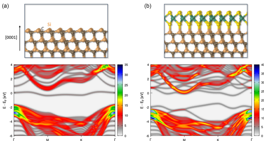
Figure 4. a) Atomic configuration of the ideal Si-terminated 4H-SiC(0001) surface (upper) and total wavevector-resolved projected density of states along the \Gamma -M-K- \Gamma Brillouin zone path (lower). b) Atomic configuration of the \text{MoS}_2 /4H-SiC(0001) interface (upper) and total wavevector-resolved projected density of states along the \Gamma -M-K- \Gamma Brillouin zone path (lower). E_F refers to the calculated Fermi level of the systems.
