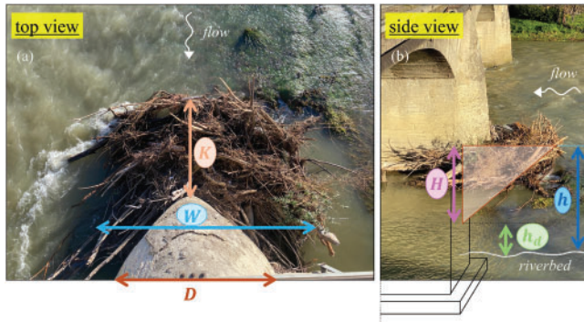
Figure 1. (a) Top-view and (b) side view of a LW accumulation at a pier, with the characteristic dimensions: the accumulation transverse width, W ; the accumulation vertical high, H ; and the accumulation upstream length, K (according to Panici and de Almeida 8 ). In the top view, the bridge pier transverse width is indicated, D . While in the side view, the sketch reports water depth upstream the bridge, h , and the distance between the riverbed and the bottom of the wood accumulation, h_d . Photographs taken by Innocenti et al. 14,31
