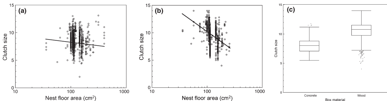
Fig. 1. Clutch size in relation to nest floor area ( \text{cm}^2 ) in (a) the great tit and (b) the blue tit, and (c) clutch size in the blue tit in wooded and concrete nest boxes. The box plot in (c) shows median, quartiles, 5- and 95-percentiles and outliers. The figures show the raw data. The lines are the linear regression lines.
