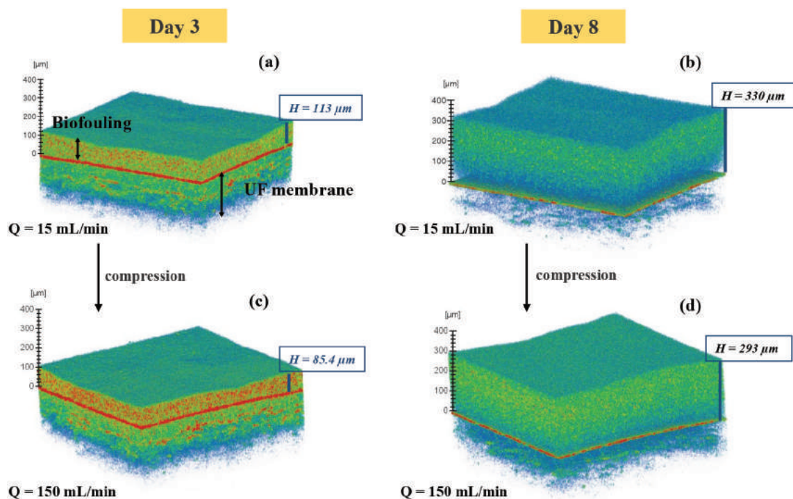
3D-visualization of biomass cake developed on UF membrane surface at Q = 15 mL/min (a, b) and under compression at Q = 150 mL/min (c, d) at various stages of biofilm growth (days 3 and 8).
