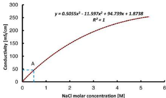
Fig. 4. Sodium chloride conductivity by varying the molar concentration.
