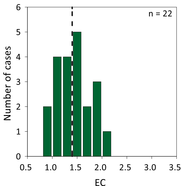
Figure 44 - Frequency distribution of EC (Log 10 ) in Mt. Soro rainwater samples (22 cases). The black dashed line is the geometric mean.
