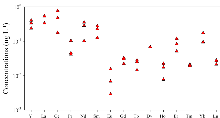
Figure 9 - Technology-Critical Elements concentrations ( \text{ng L}^{-1} ) in the blank solutions.
