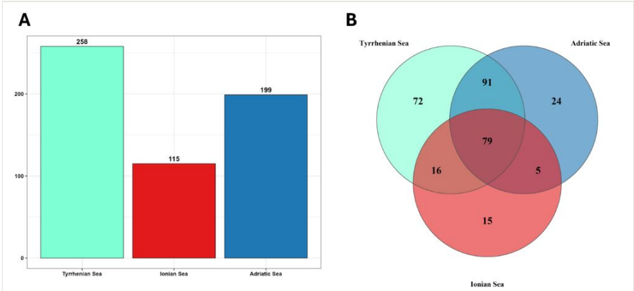
Figure 4. A Number of species per sea; B Venn diagram illustrating the distribution and shared amphipod species across the three areas, Tyrrhenian Sea (light blue), Ionian Sea (red), Adriatic Sea (blue).
