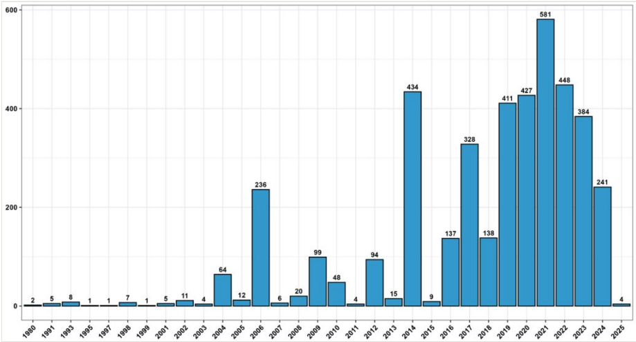
Figure 2. Graph showing the distribution of records through the years from 1980 to 2025.
