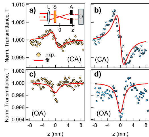
FIG. 3. Z-scan Traces. (a, b) Closed and (c, d) open aperture Z-scan data for free-standing (a, c) pristine and (b, d) patterned SiN membranes with I_0 = 720 GW/cm 2 (a, b), I_0 = 1017 GW/cm 2 (c), and I_0 = 650 GW/cm 2 (d). A theoretical profile (red solid line) based on Ref. 19 has been fitted to the measured data (markers). The inset sketches the Z-scan setup. The position z = 0 denotes the beam focus. L: lens; S: sample; A: aperture; D: detector. The data in (a) and (b) have been measured with S = 0.495 and S = 0.485 , respectively.
