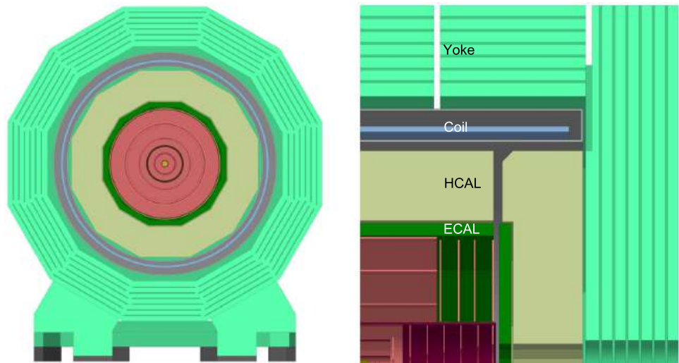
Fig. 92 The CLD concept detector: end-view cut through (left) and longitudinal cross section of the top right quadrant (right). The detector has an overall diameter of 12.0 m and an overall length of 10.6 m
