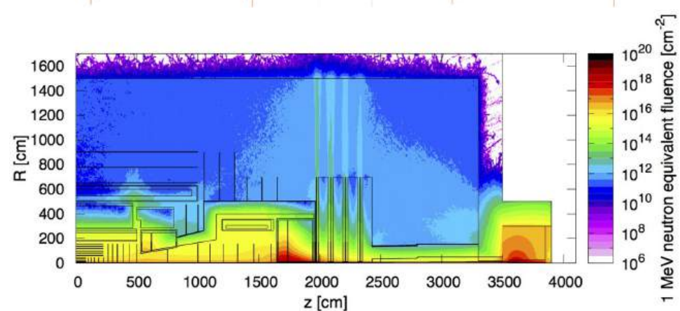
Fig. 123 Total radiation load for the FCC-hh detector and the final focusing magnets in the machine tunnel, with a possible ultimate integrated luminosity of 30 \text{ ab}^{-1}
