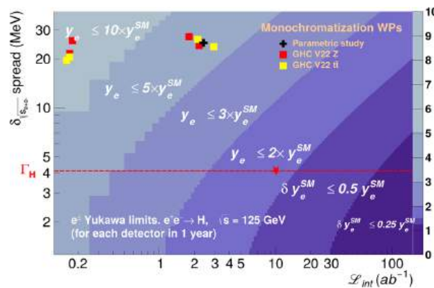
Fig. 137 Upper limit contours (at 95% CL) on the electron Yukawa y_e (coloured bands) in the collision-energy spread \delta\sqrt{s} vs. integrated luminosity \mathcal{L}_{int} plane. The red star over the \delta\sqrt{s} = \Gamma_H = 4.1 MeV red-dashed line indicates the reference point assumed in the physics simulation analysis [32]. The black cross indicates the previously achieved working point with self-consistent parametric monochromatisation [839,842]. The red and yellow squares indicate the monochromatisation points based on simulations of the ‘GHC V22 Z’ and ‘GHC V22 t’ optics, respectively (see text for details) [843]
