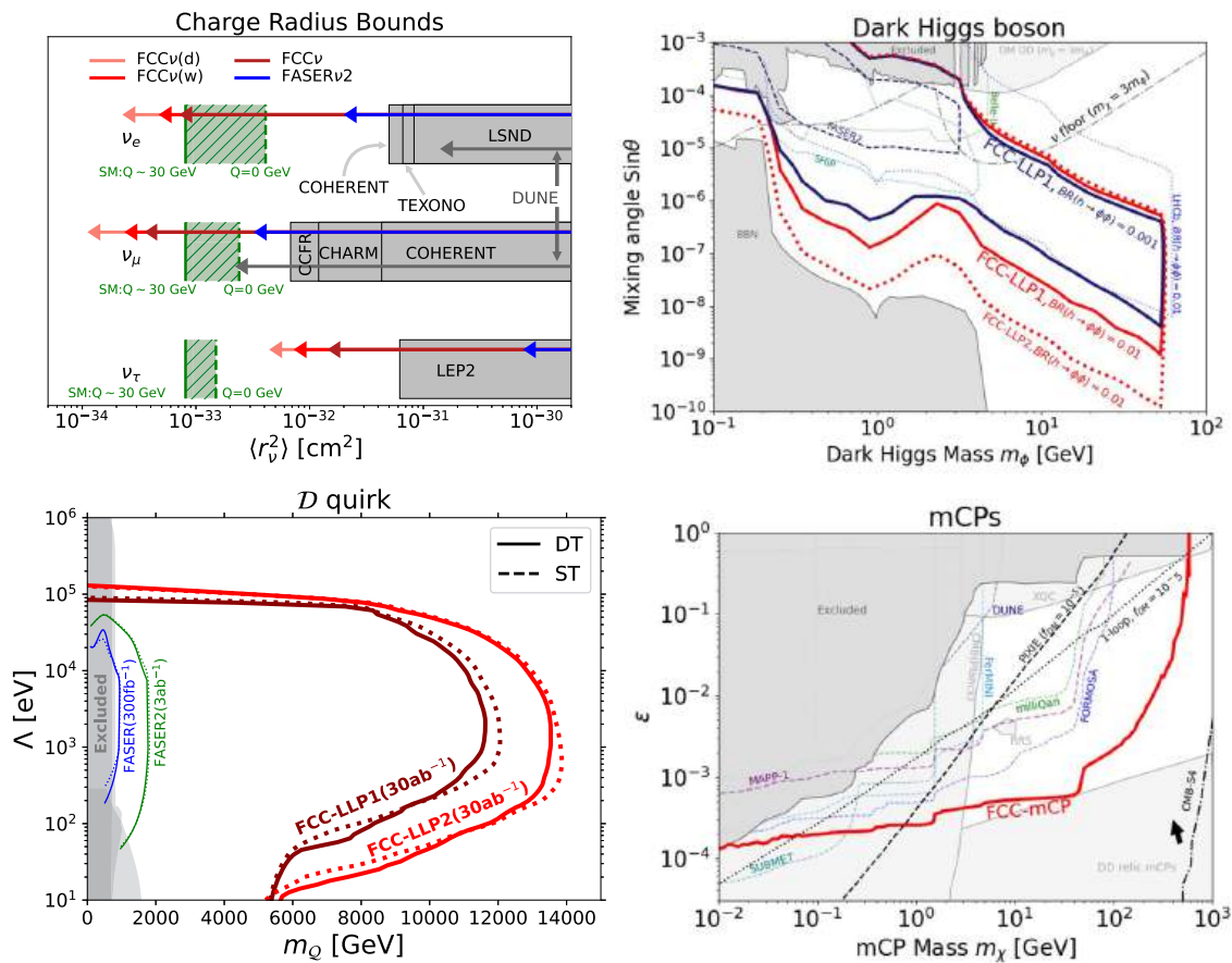
Fig. 46 Top left: sensitivity of the FCCν detectors to the neutrino charge radius. Top right: reach for a dark Higgs boson \phi at the PPF@FCC. Bottom left: discovery potential for D -type quarks with mass m_Q and confinement scale \Lambda . Bottom right: Sensitivity to mCPs with mixing parameter \epsilon
