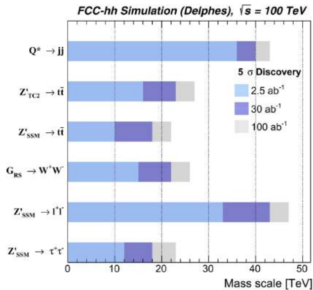
Fig. 32 Summary of the 5\sigma discovery reach, as a function of the resonance mass, for different FCC-hh luminosity scenarios. From Ref. [190]
