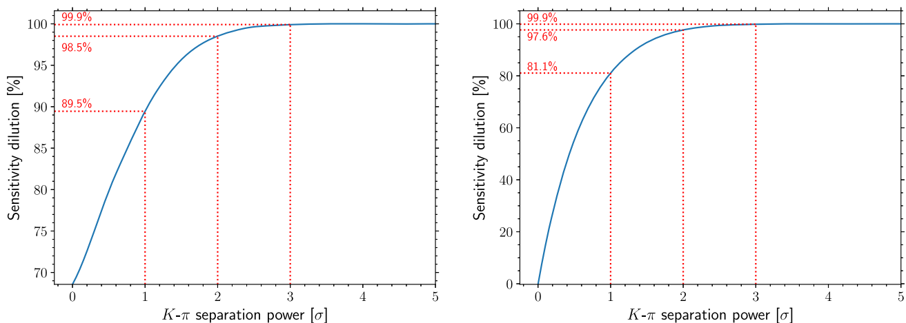
Fig. 58 Sensitivity to the B \rightarrow K^* \nu \bar{\nu} (left) and B_s \rightarrow \phi \nu \bar{\nu} (right) branching fractions, as a function of the \pi/K separation power, with respect to the sensitivity assuming perfect PID
