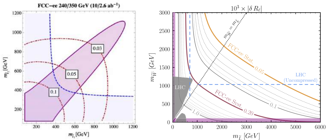
Fig. 27 Left: projected 2\sigma sensitivity of Higgs couplings to stops at FCC-ee in the parameter space of stop masses m_{t_1} vs. m_{t_2} ; from Ref. [116]. Right: FCC-ee Z branching ratio projected statistical and
