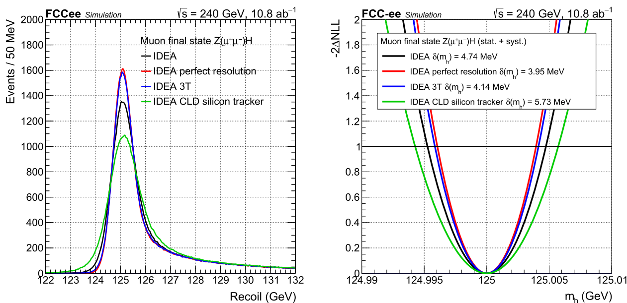
Fig. 48 Left: fits to the distribution of the Higgs boson recoil mass in ZH events, where the Z decays into muons, assuming an ideal momentum resolution (red), such that the resolution on the recoil mass is determined by the beam energy spread, or the momentum resolution of the
