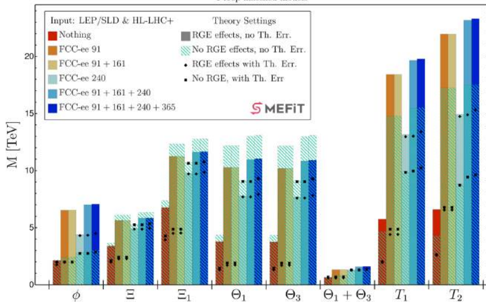
Fig. 21 Sensitivity (95% CL) to a selection of models from Table 4 with Wilson coefficients fully matched at one-loop (the bounds are obtained from a \chi^2 fit and the couplings of the new particle are set to unity at the matching scale, taken to be the mass of this heavy particle, the different operators are then run down to the Z boson mass with full numerical resummation of the logarithmic terms). In the case of new physics coupled to SM fermions, heavy scalar and fermions couple to the
