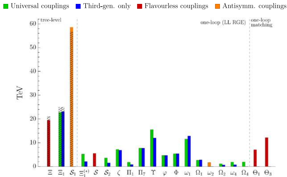
Fig. 18 Projected bounds on the masses of new scalar fields (the bounds are 2\sigma fits, obtained running with the leading-logarithmic terms from a scale of 2 TeV, at which the couplings to the SM particles are assumed to be unity, down to the mass of the Z). ‘Flavourless couplings’ correspond to models in which couplings of the new states to fermions are absent, ‘Universal couplings’ correspond to equal couplings to all
