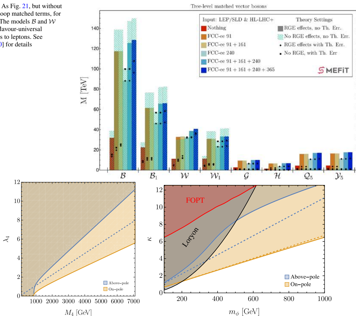
Fig. 25 FCC-ee sensitivity at 68% CL on the weak custodial quadruplet scalar (left) and real singlet scalar (right) models in the mass vs. coupling plane when combining Z pole data (orange) with ZH measure-
