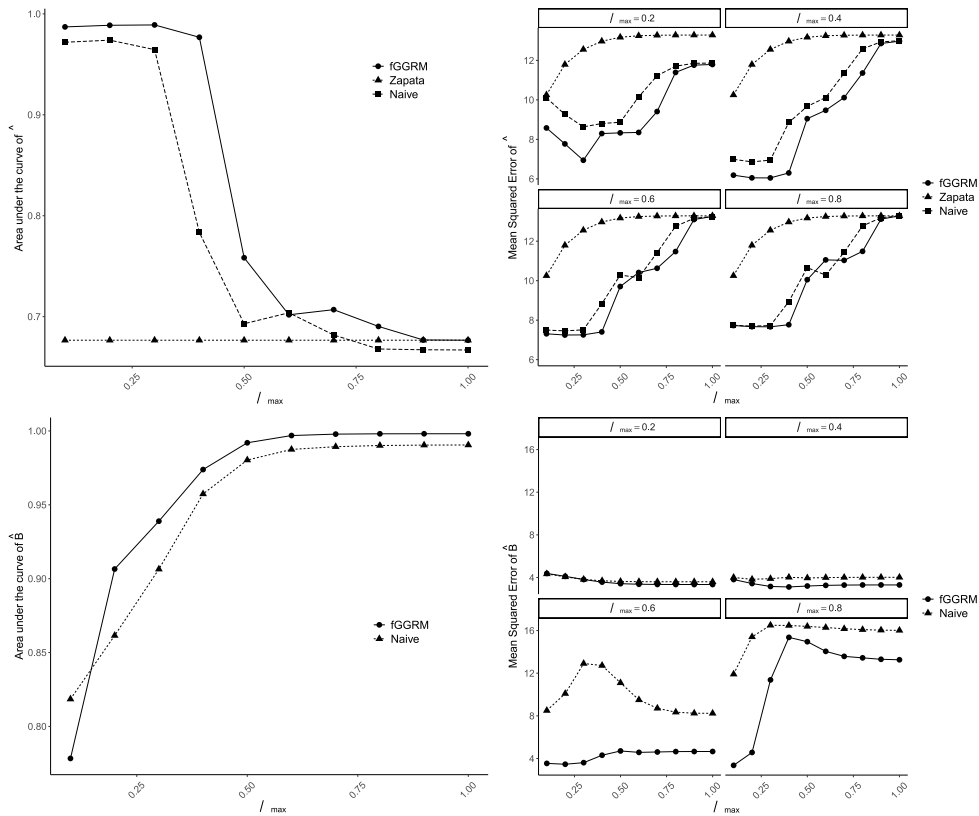
Figure 7. Simulation results for N = 50 , p = 100 , and q = 10 . The upper panels compare fGGRM with the method in Zapata et al. (2021) and a naive estimator. The lower panels omit the method from Zapata et al. (2021) since it does not account for functional predictors. The left panels report AUC curves for the edge sets \mathcal{E}^V and \mathcal{E}^{X^V} , while the right panels present MSE curves for \Theta_l and B_l . AUC values are plotted against the ratios \nu \nu_{\max} and \rho \rho_{\max} , while MSE curves for \Theta_l and B_l are computed over ten values of \rho and \nu , respectively, keeping the regression and precision matrix structures fixed at selected ratios of \nu \nu_{\max} and \rho \rho_{\max} .
