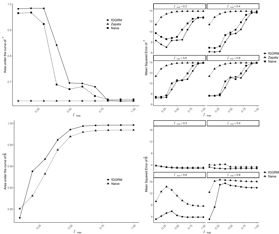
Figure 8. Simulation results for N = 50 , p = 100 , q = 10 , and c = 0.1 . The upper panels compare fGGRM with the method in Zapata et al. (2021) and a naive estimator. The lower panels omit the method from Zapata et al. (2021) since it does not account for functional predictors. The left panels report AUC curves for the edge sets \mathcal{E}^Y and \mathcal{E}^{XY} , while the right panels present MSE curves for \Theta_l and B_l . AUC values are plotted against the ratios v/v_{\max} and \rho/\rho_{\max} , while MSE curves for \Theta_l and B_l are computed over ten values of \rho and v , respectively, keeping the regression and precision matrix structures fixed at selected ratios of v/v_{\max} and \rho/\rho_{\max} .
