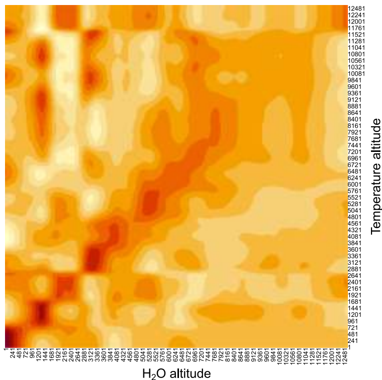
Figure 10. Regression function values \beta_{\text{H}_2\text{O}}(t, s) for all t, s = 1, \dots, 420 . The x-axis represents \text{H}_2\text{O} altitude, while the y-axis represents temperature altitude. Darker regions denote the highest regression values (0.00025), while lighter regions indicate the lowest values (−0.00006).
