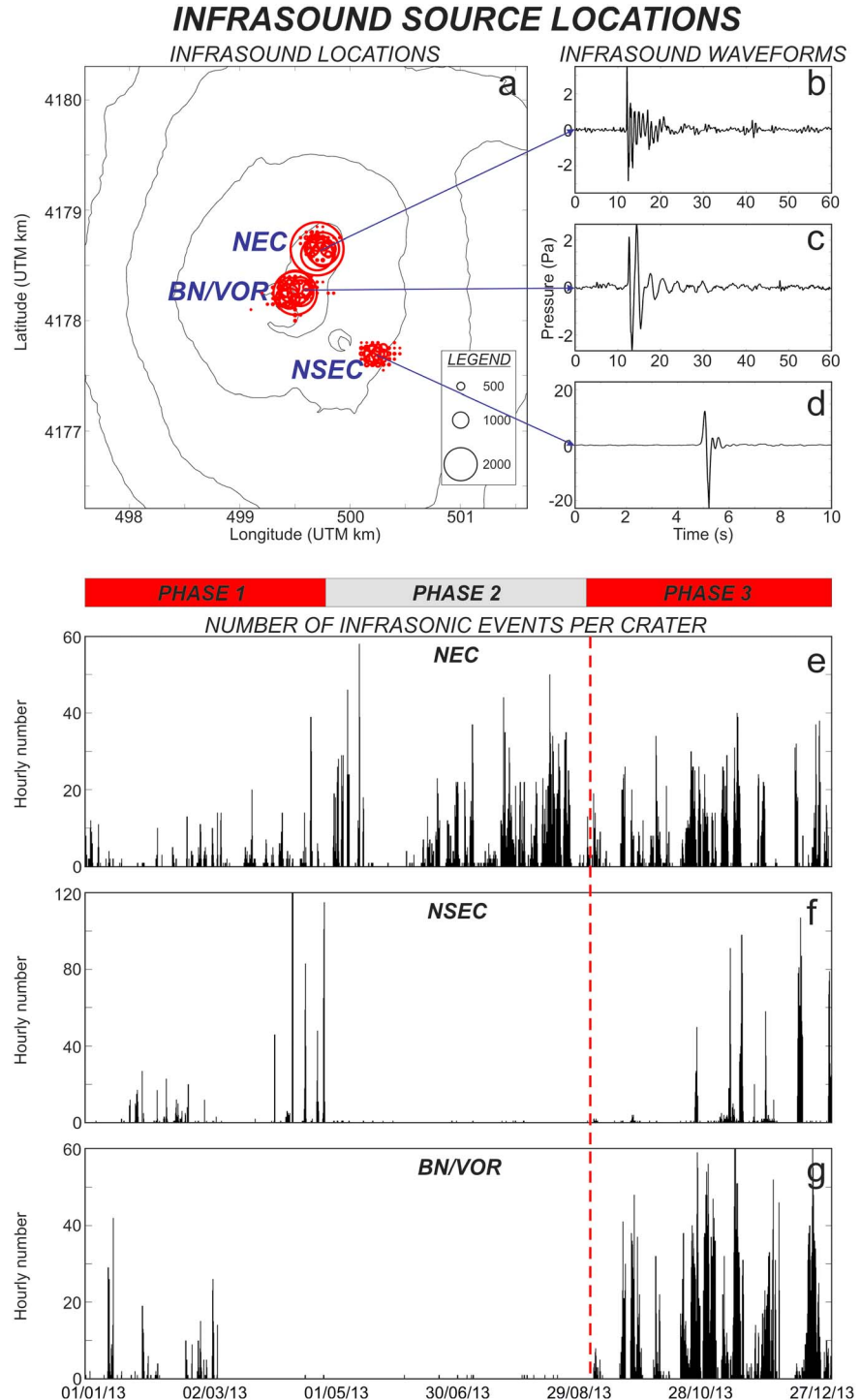
Figure 8. Infrasound source locations. (a) Map of Etina with the location of the infrasonic events recorded during 2013 (the radii of the red circles are proportional to the number of locations of infrasonic events in each grid node; see legend in the bottom right corner). (b–d) Waveforms of typical infrasonic events generated by NEC, BN, and NSEC, respectively. (e) Hourly number of infrasonic events located in the NEC area during 2013. (f) Hourly number of infrasonic events located in the NSEC area during 2013. (g) Hourly number of infrasonic events located in the BN/VOR area during 2013. The vertical dashed red line in Figures 8e–8g indicates the occurrence time of the explosion at BN, which took place on 5 September 2013 at 15:39. The top red and grey rectangles indicate the time intervals called Phase 1, Phase 2, and Phase 3 (see section 4 for details).
