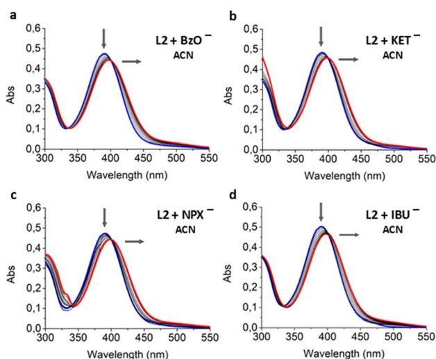
Fig. 9 UV-Vis titrations performed in ACN of L2 with the gradual addition (0–10 eq.) of (a) BzO − , (b) KET − , (c) NPX − , (d) IBU − [ L2 ] = 1 × 10 −5 mol dm −3 . In all of the experiments, blue lines refer to the spectrum of the free ligands and red lines to the spectrum registered after the last addition of the anion.
