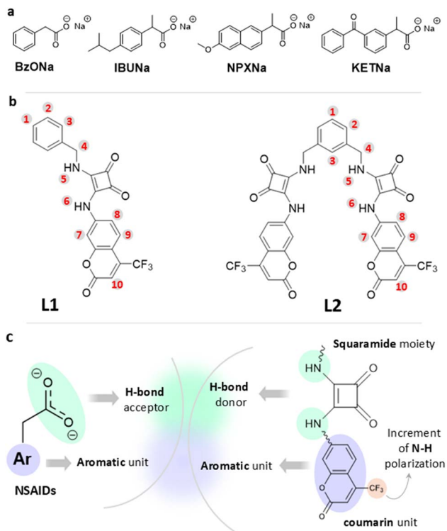
Fig. 1 (a) Molecular structures of the NSAIDs and benzoate sodium salts studied in this paper; (b) structures of ligands L1 and L2 together with ^1\text{H} NMR labelling; and (c) schematic for the ligand design.
