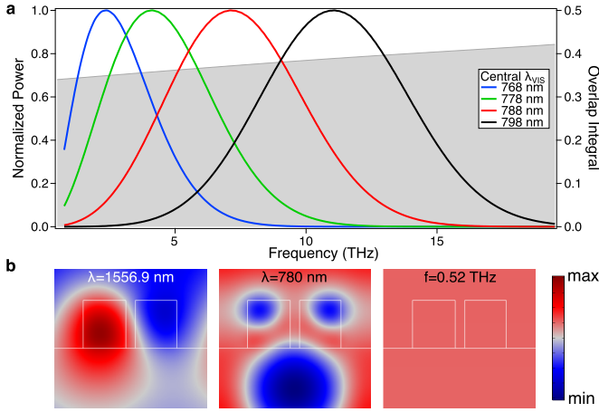
Fig. 3. a. Frequency-resolved power spectra (normalized units) of the output THz radiation for different values of \lambda_{VIS} . The shaded area corresponds to the overlap integral. b. Selected field profiles employed for the overlap integral calculation.
