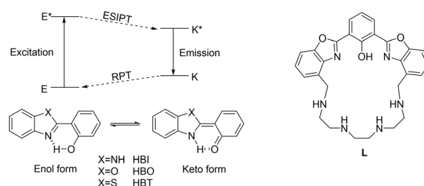
Fig. 1 Left: the schematic of the ESIPT and the RPT processes in 2-(2-hydroxyphenyl)benzimidazole (HBI), 2-(2-hydroxyphenyl)benzoxazole (HBO) and 2-(2-hydroxyphenyl)benzothiazole (HBT). 8 Right: the structure of the ligand L , containing the bis-HBO fluorophore.
