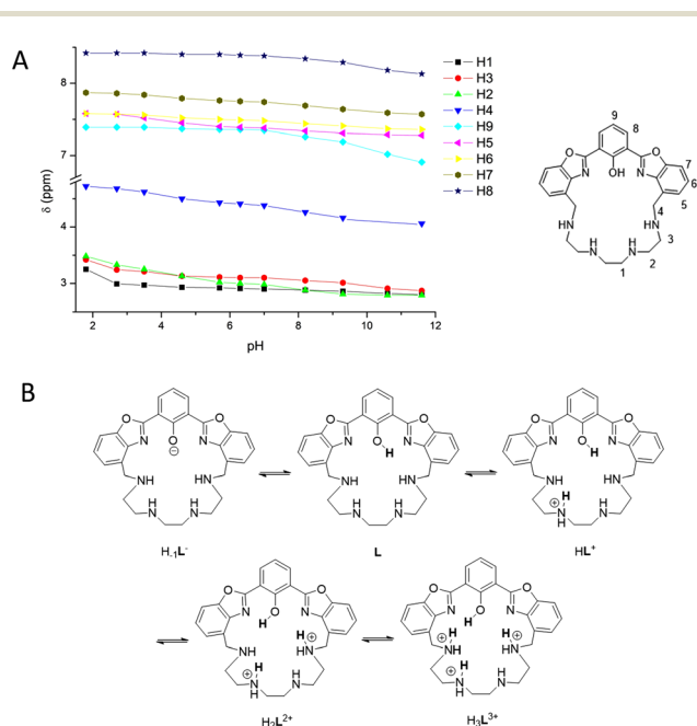
Fig. 4 (A) Trend of the ^1\text{H} -NMR signals of L as a function of pH. Proton labels are shown in the structure on the right. (B) Proposed disposition of acidic protons in the species from \text{H}_{-1}\text{L}^- to \text{H}_3\text{L}^{3+} .
