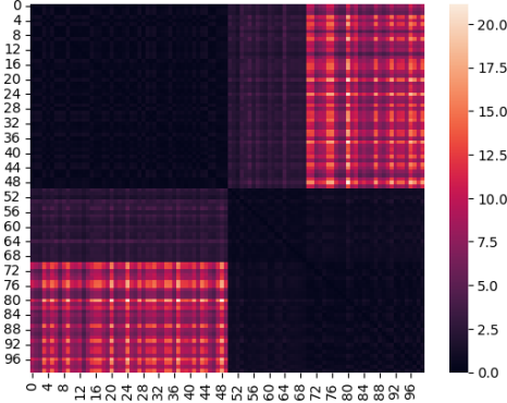
(c) 50% malicious, low noise
