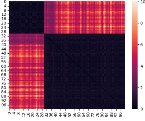
(a) 30% malicious, low noise
