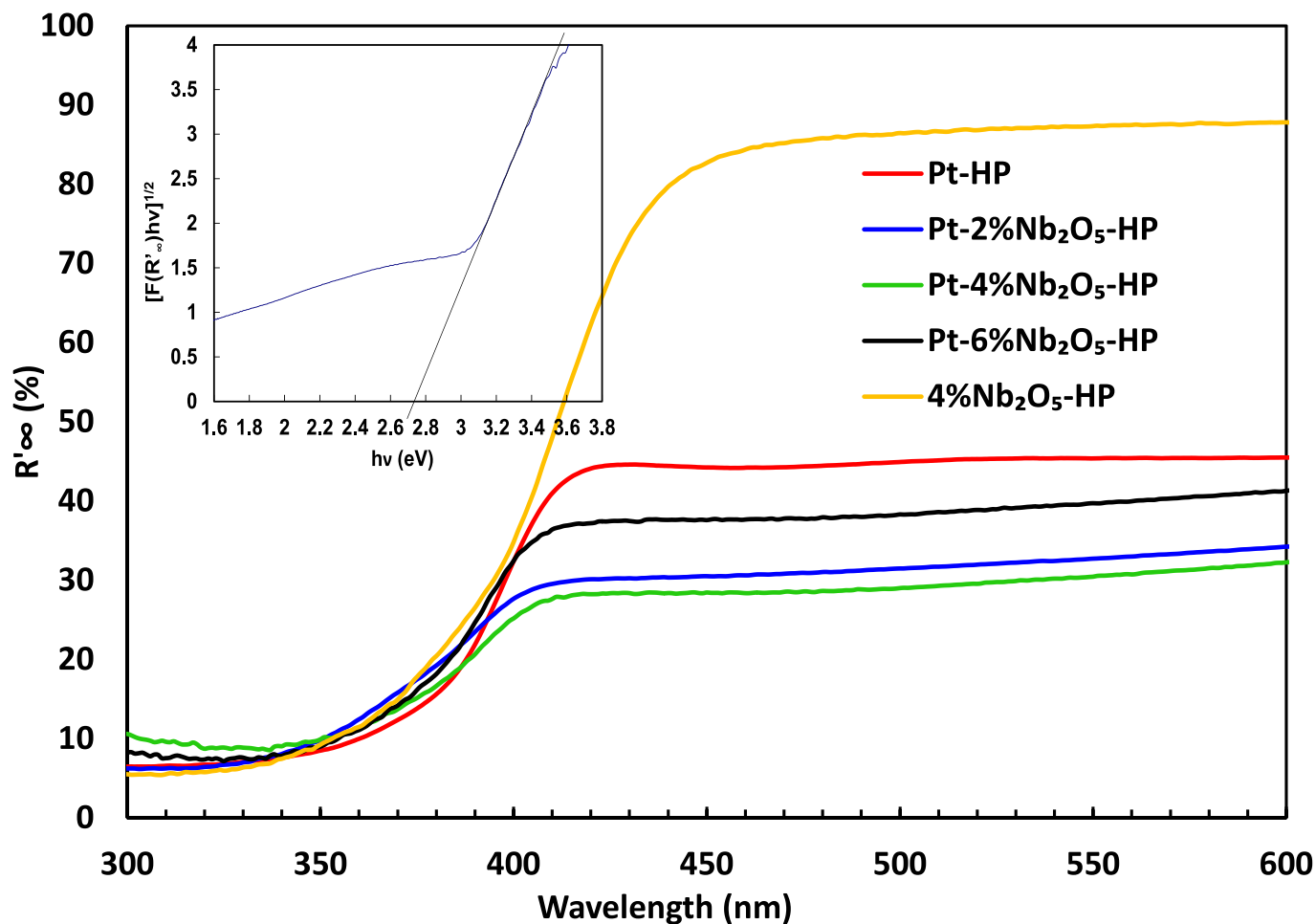
Fig. 2. UV-Vis DRS spectra of the prepared photocatalysts.
