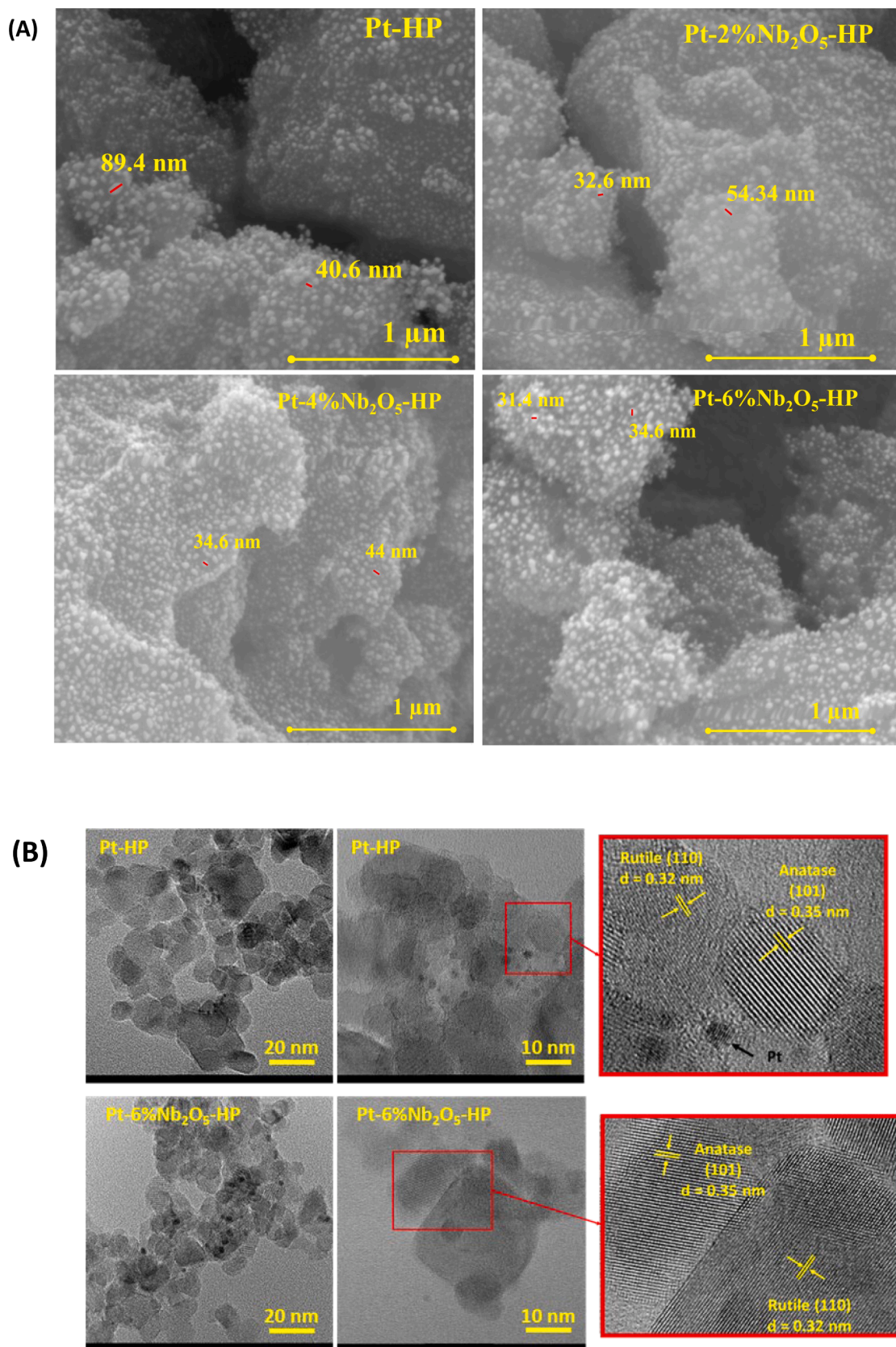
Fig. 8. Selected SEM micrographs of the examined photocatalysts (A); TEM images of the Pt-HP and Pt-6 %Nb 2 O 5 -HP samples (B).
