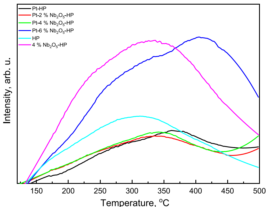
Fig. 7. Pyridine TPD curves for the investigated photocatalysts.
