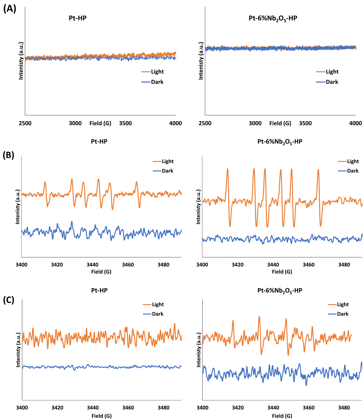
Fig. 10. EPR spectra of (A) powder samples Pt-HP and Pt-6 %Nb 2 O 5 -HP under dark and light irradiation, (B) samples suspended in H 2 O/DMPO/MeOH solution, and (C) samples suspended in H 2 O/DMPO/H 2 O 2 solution.
