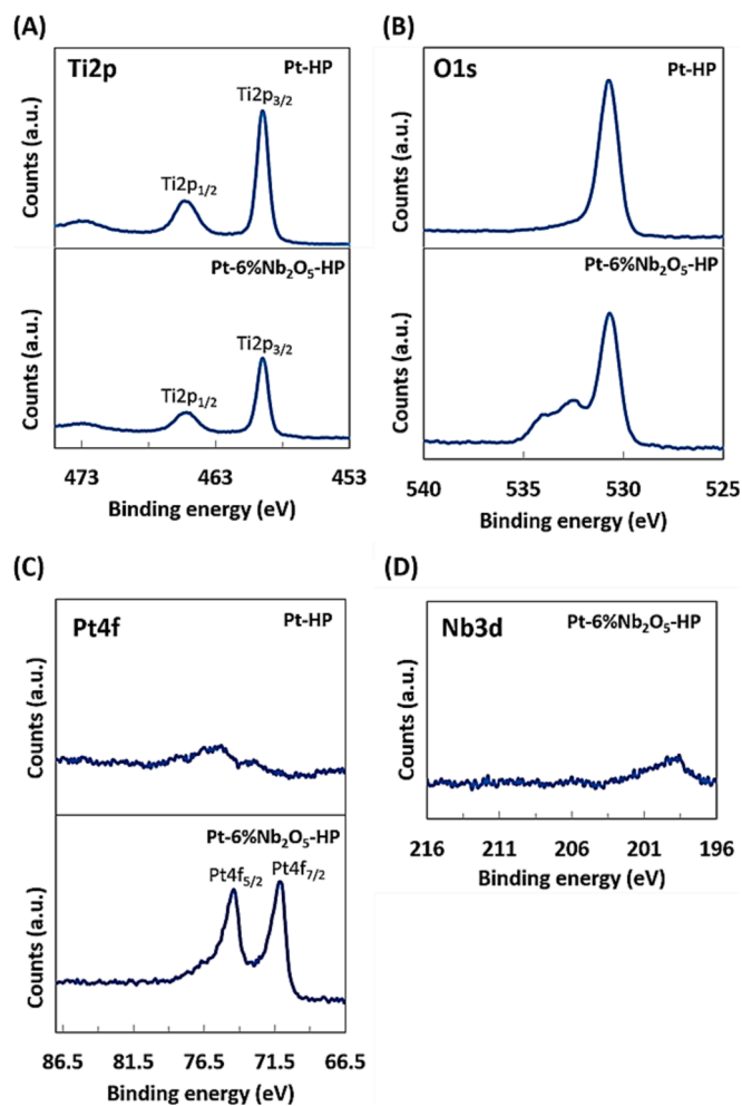
Fig. 9. High resolution XPS spectra of (A) Ti 2p, (B) O 1 s, (C) Pt 4f, and (D) Nb 3d peaks.
