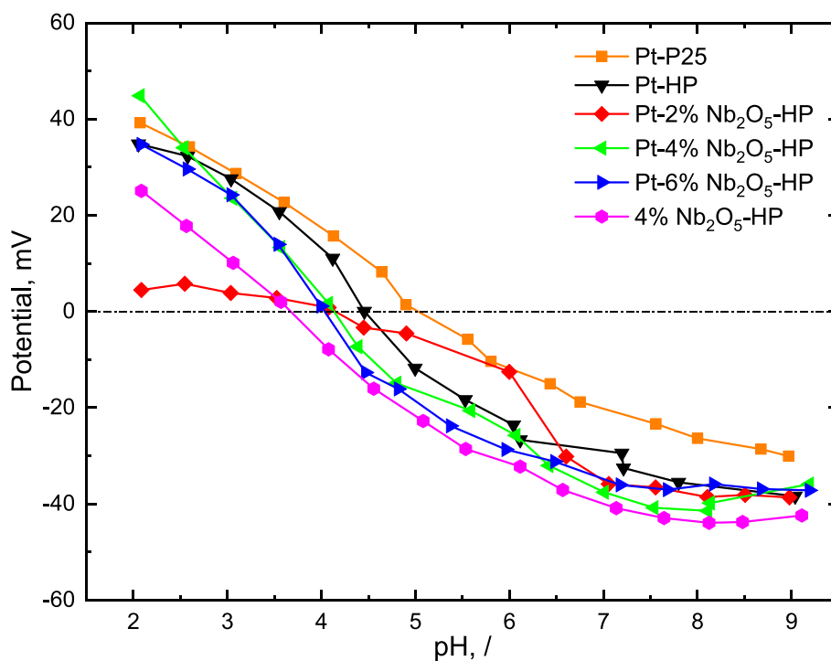
Fig. 3. Results of the pH related zeta potential measurements.
