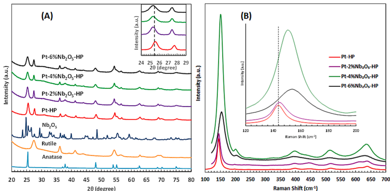
Fig. 1. XRD patterns (A) and Raman spectra (B) of Anatase, Rutile, Nb 2 O 5 , Pt-HP, Pt-2 %Nb 2 O 5 -HP, Pt-4 %Nb 2 O 5 -HP and Pt-6 %Nb 2 O 5 -HP samples.
