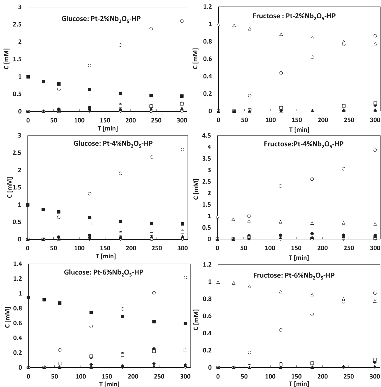
Fig. 11. Concentrations of the two substrates and their products versus irradiation time for runs carried out by using Nb 2 O 5 modified photocatalysts. Legend: ■ glucose, Δ fructose, ● arabinose, ◇ gluconic acid, □ formic acid, ○ hydrogen, ▲ CO 2 .
