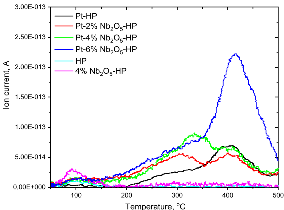
Fig. 5. CO 2 TPD curves of tested materials.
