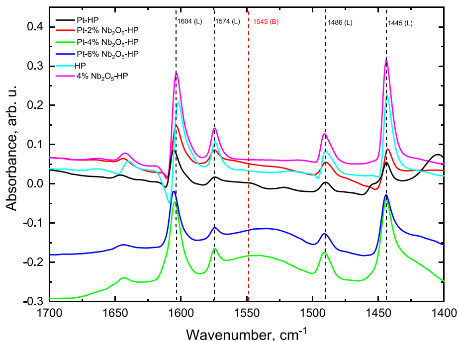
Fig. 6. DRIFTS spectra of pyridine adsorbed on the surface of investigated materials.
