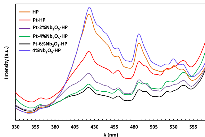
Fig. 4. Solid-state photoluminescence spectra of the different samples.
